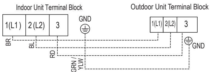
Figure 38: Indoor Unit to Outdoor Unit Power Wiring / Communications Cable Connections.
