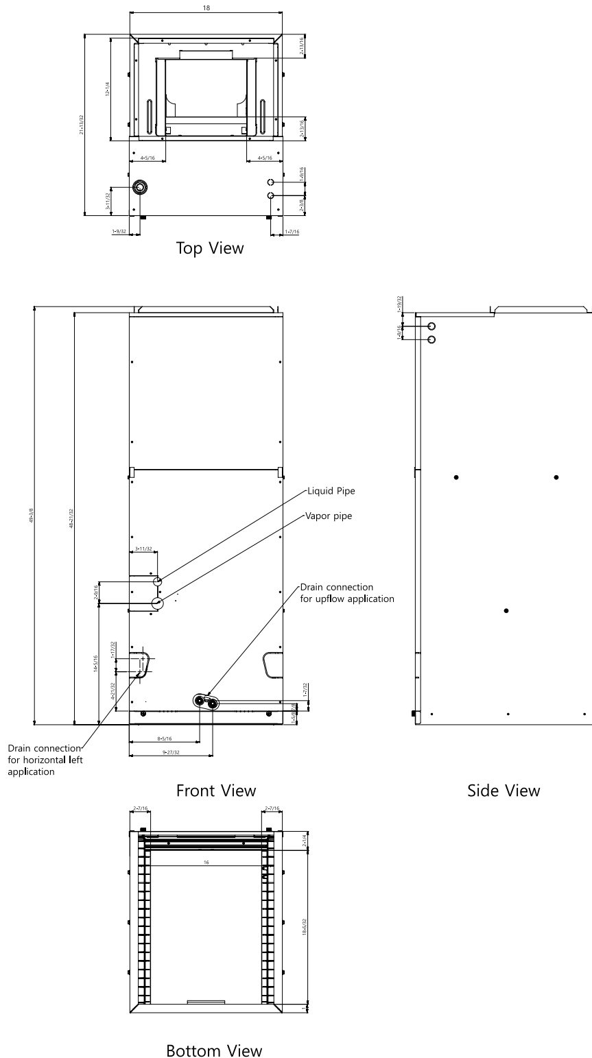
Figure 6: LVN181HV4, LVN241HV4, LVN361HV4 Indoor Unit Dimensions.
