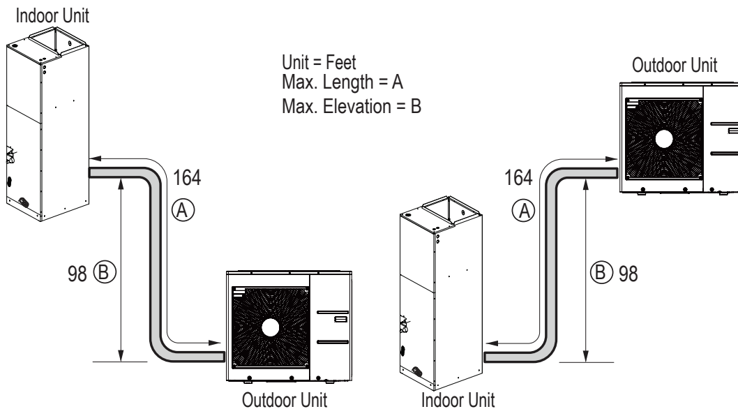
Figure 63: Typical LV181HV4 and LV241HV4 System Layout.
