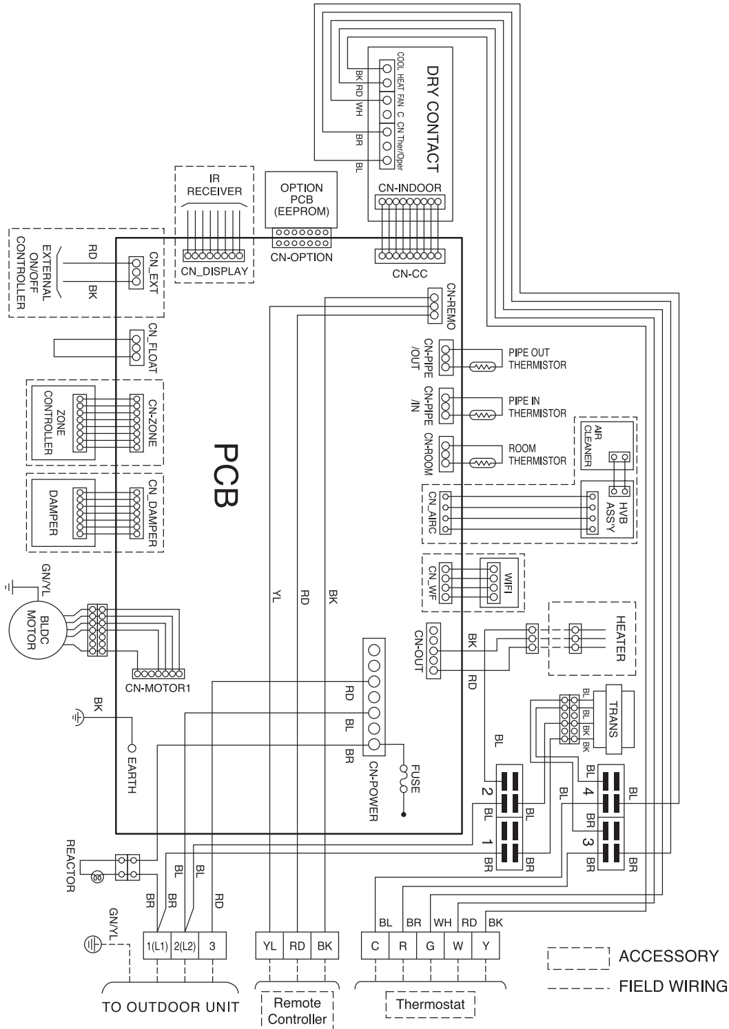
Figure 29: Indoor Unit Wiring Diagram.
