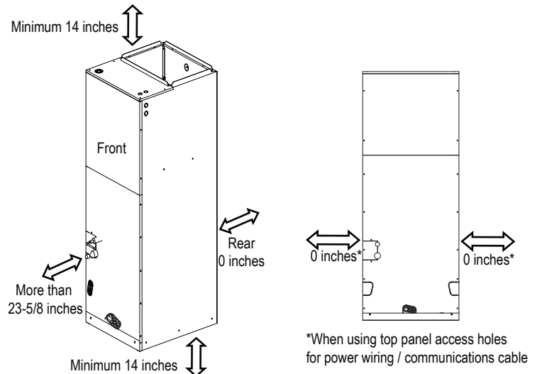
Figure 50: Recommended Clearances for Vertical Air Handler Unit IDU.
