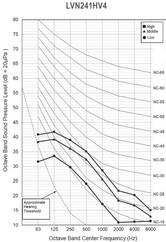
Figure 10: LVN241HV4 Sound Pressure Level Diagram.
