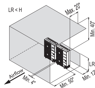
Figure 61: Proper Outdoor Unit Placement and Clearances, continued.
