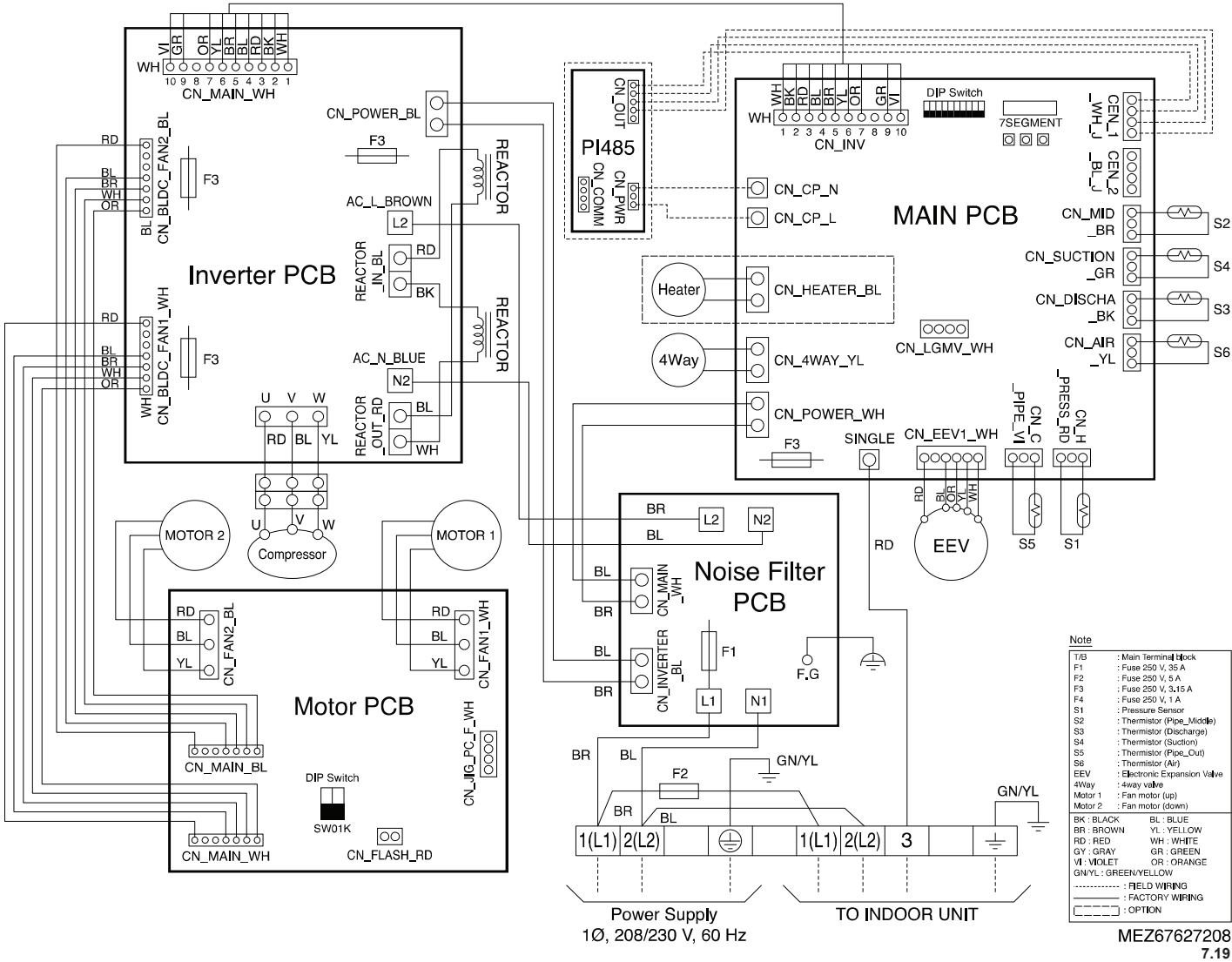
Figure 32: Outdoor Unit Wiring Diagram.
