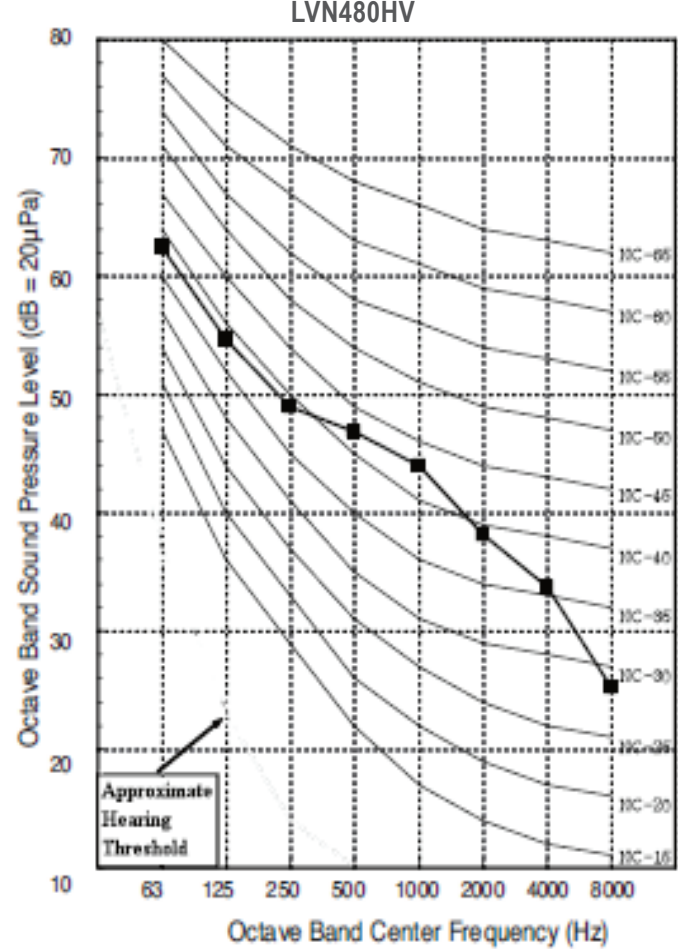
Figure 13: LVN480HV Sound Pressure Level Diagram.
