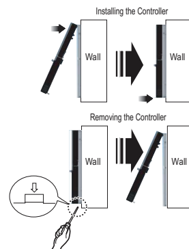
Figure 44: Installing / Removing the Controller.
