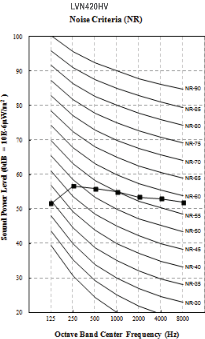
Figure 17: LVN420HV Sound Power Level Diagram.
