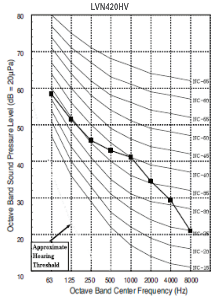
Figure 12: LVN420HV Sound Pressure Level Diagram.
