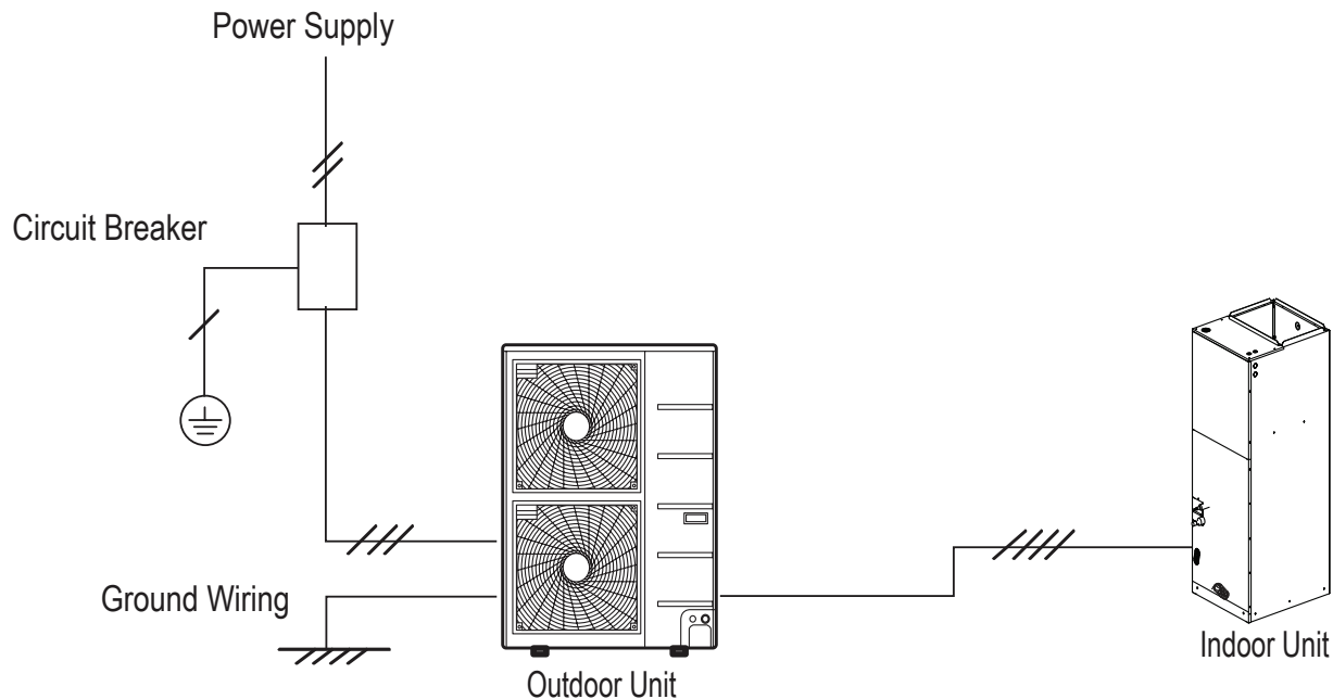
Figure 36: LV361HV4, LV480HV, and LV488HV General Power/Communications System Schematic.
