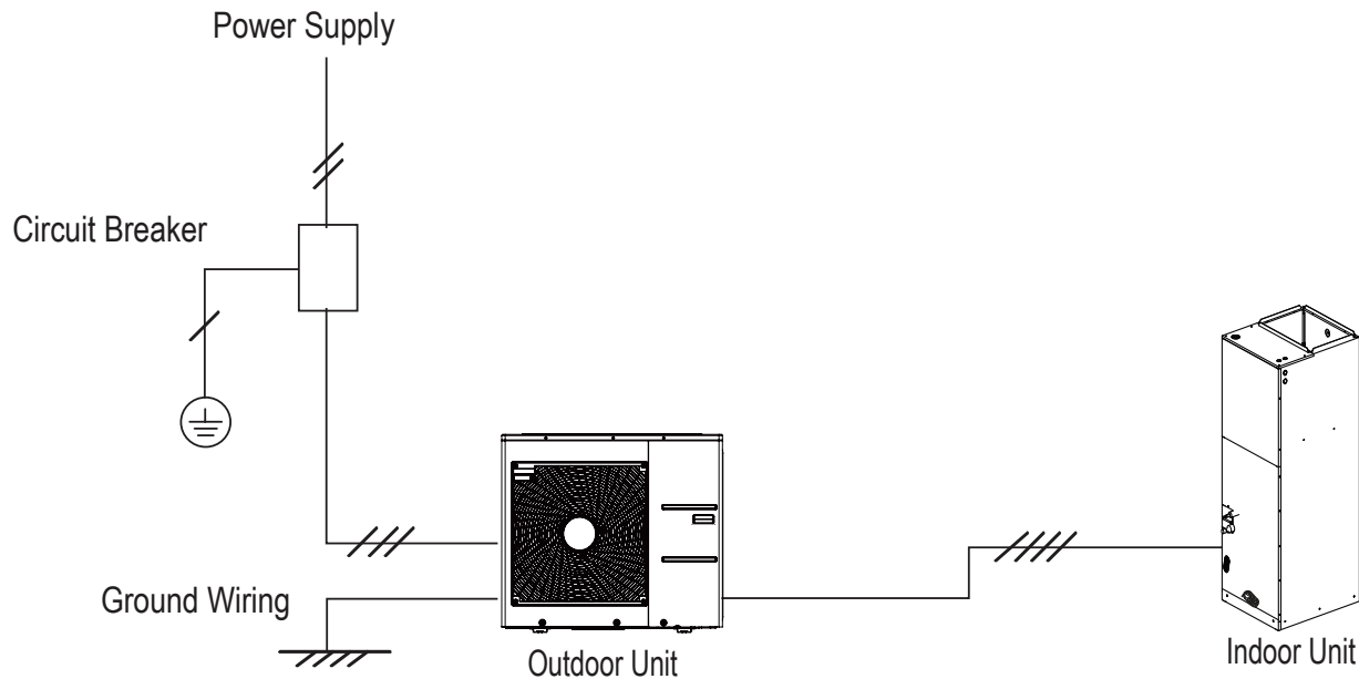
Figure 36: LV361HV4, LV480HV, and LV488HV General Power/Communications System Schematic.
