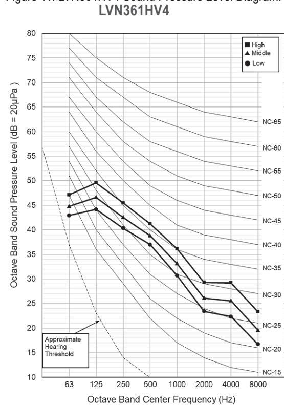
Figure 11: LVN361HV4 Sound Pressure Level Diagram.
