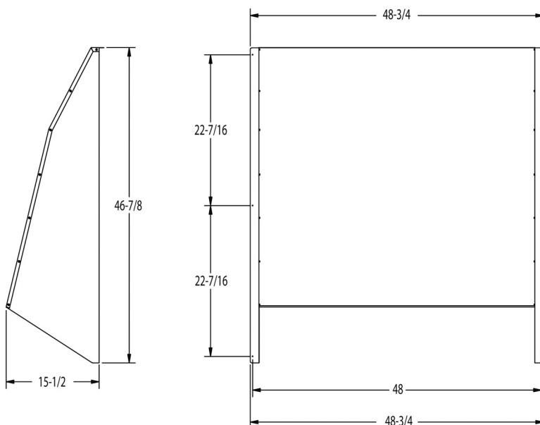
Rear Hail Guard
