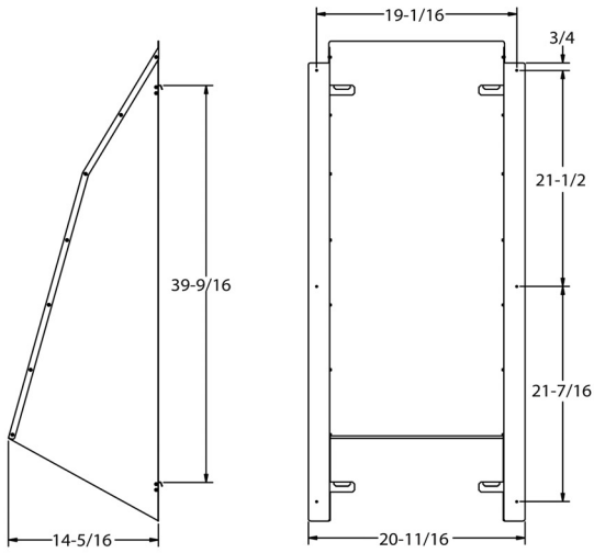
Left Hail Guard
