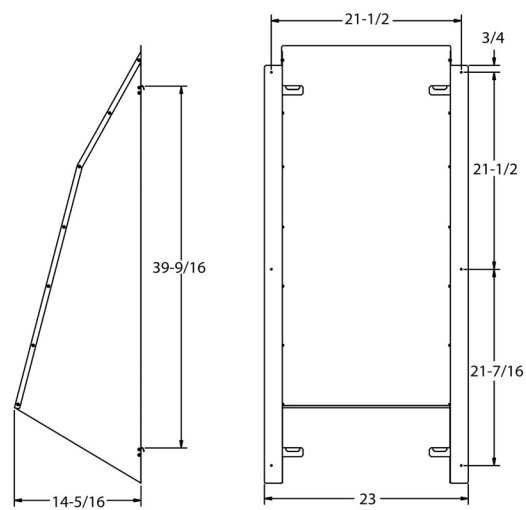
Right Hail Guard
