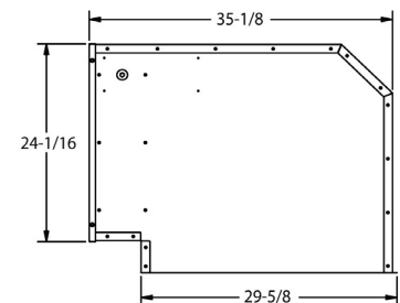
Left Top Discharge Elbow
