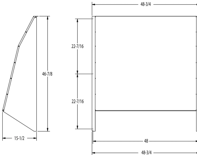
Rear Wind Baffle
