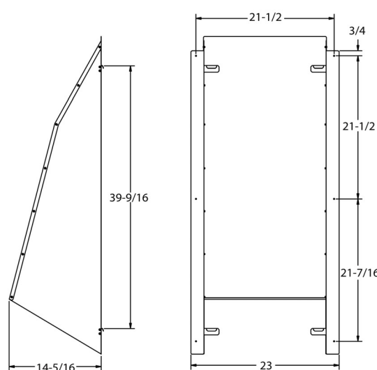
Right Wind Baffle
