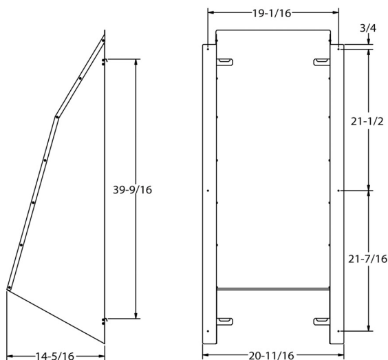
Left Wind Baffle
