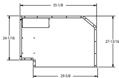
Right Top Discharge Elbow
