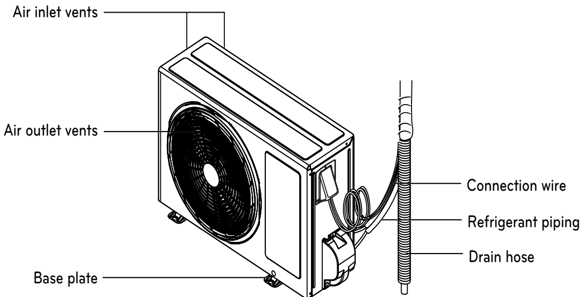
Figure 2: Outdoor Unit Basic Components
