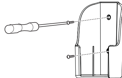
Figure 6: Holder Attachment
