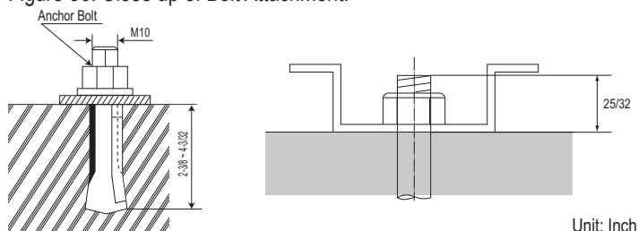
Figure 36: Close up of Bolt Attachment.
