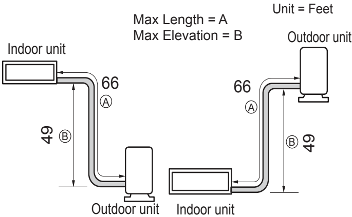
Figure 38: Typical LQ090HV4, LQ120HV4 System Layout.
