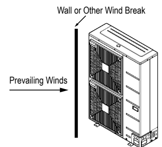
Figure 31: Wind Break.
