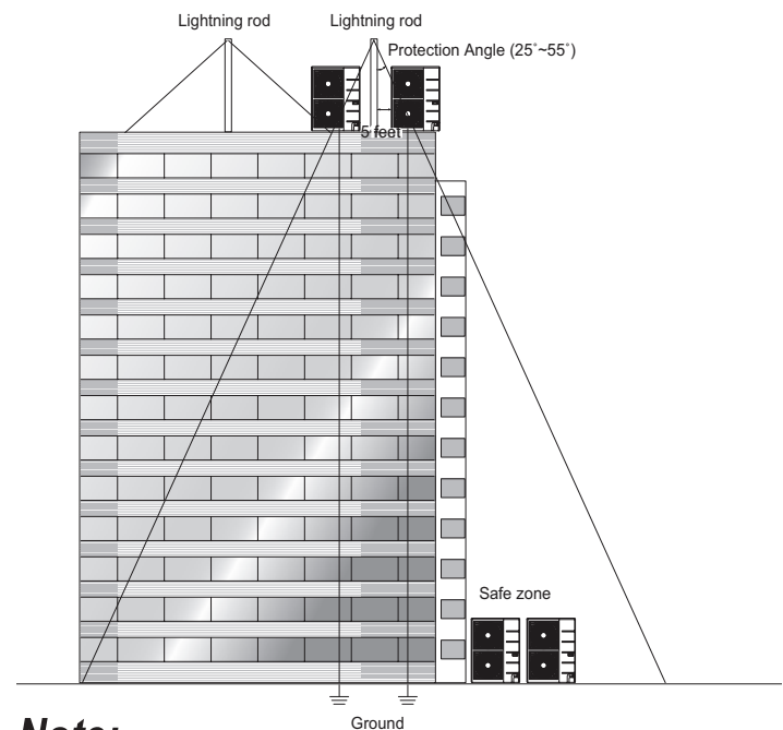
Figure 27: Lightning Protection Diagram.
