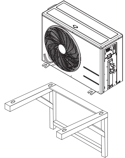
Figure 33: Bracket Mounting.
