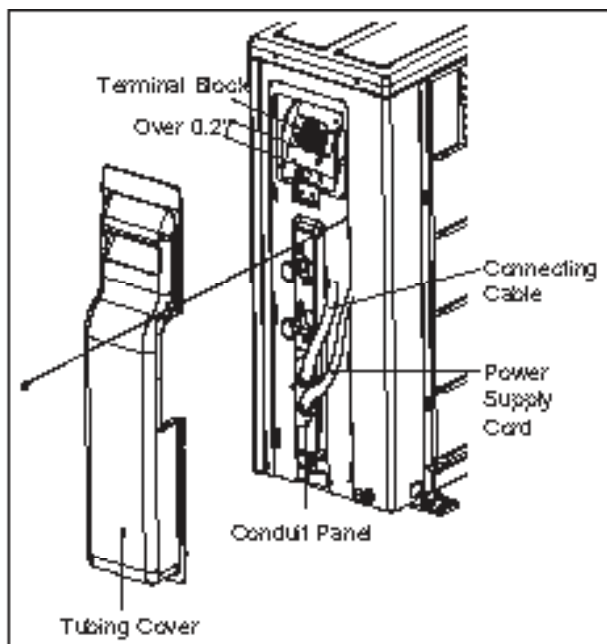
Figure 16: LUU097HV, LUU127HV ODU Terminal Block Location.
