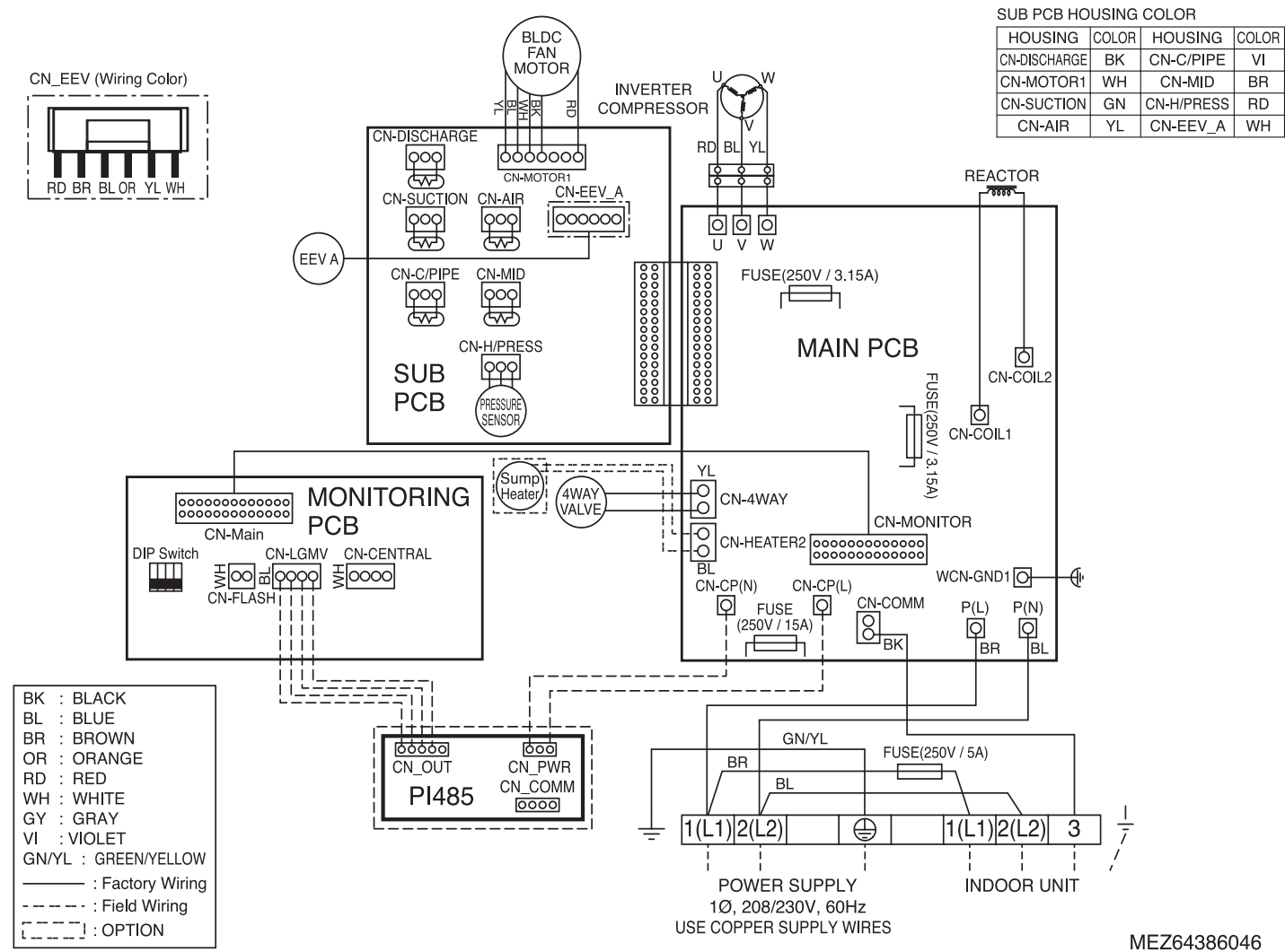
Figure 14: LUU097HV and LUU127HV Outdoor Unit Wiring Diagram.
