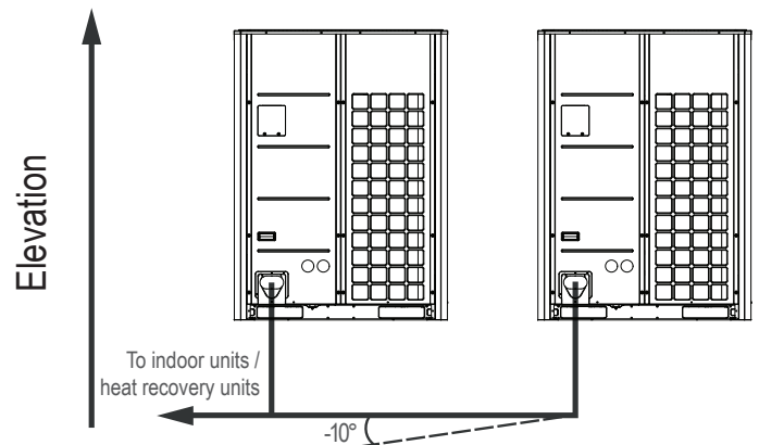
Figure 32: Allowable Pipe Slope.
