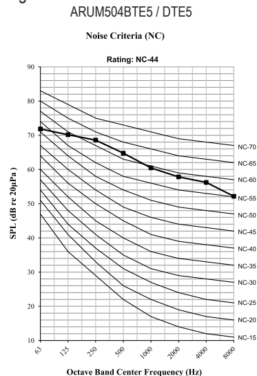
Figure 10: ARUM504BTE5 / DTE5 Sound Pressure Levels.
