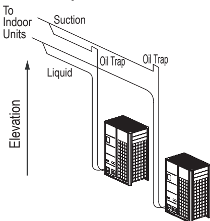
Figure 28: Traps for Heat Pump and Heat Recovery Systems.
