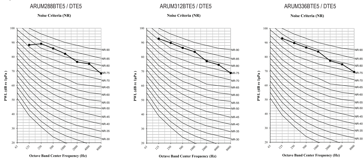
Figure 14: ARUM288-312-336BTE5 / DTE5 Sound Power Levels.
