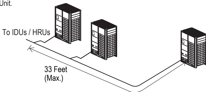
Figure 26: Maximum Pipe Length from First Outdoor Unit Y-branch to Farthest Outdoor Unit.
