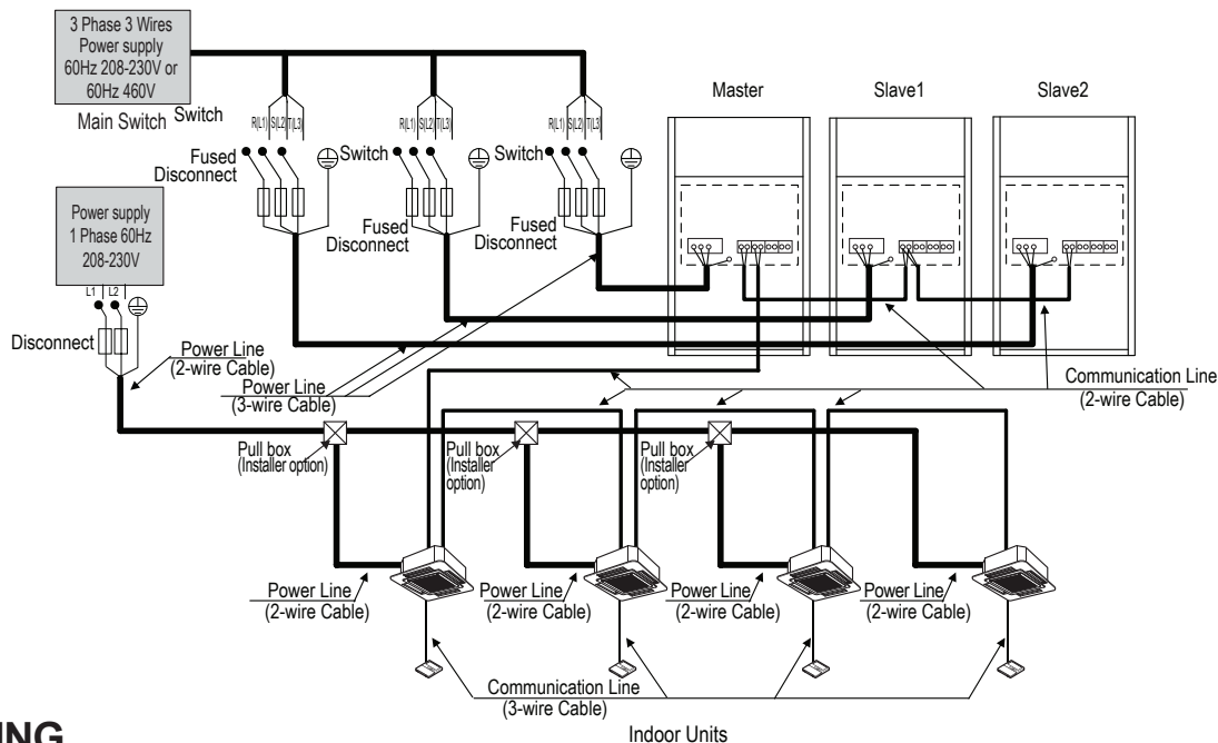
Figure 19: Example of a Typical Heat Pump Operation Power Wiring and Communications Cable Schematic.
