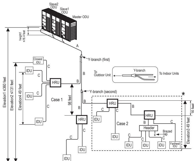
Figure 24: Heat Recovery Triple Frame Connections.
