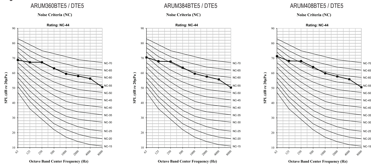
Figure 9: ARUM432-456-480BTE5 / DTE5 Sound Pressure Levels.
