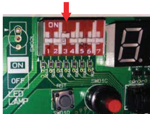
Figure 21: Location and Setting of Outdoor Unit DIP Switch 3.
