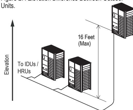
Figure 27: Elevation Difference Between Outdoor Units.
