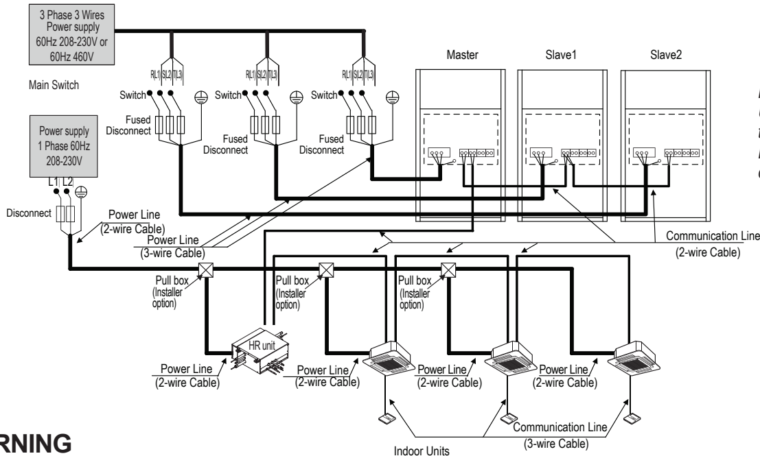
Figure 20: Example of a Typical Heat Recovery Operation Power Wiring and Communications Cable Schematic.
