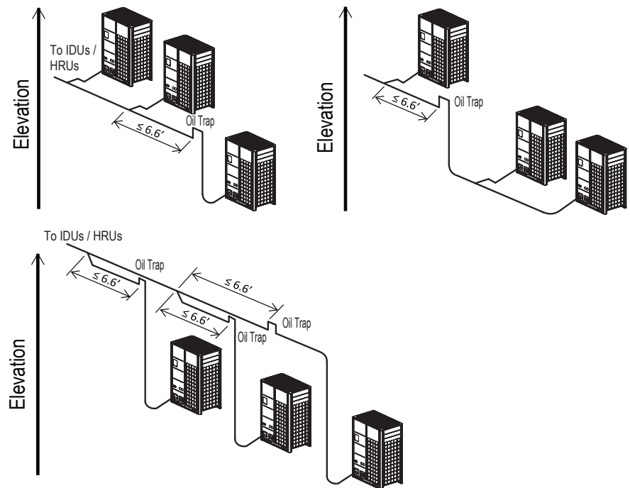
Figure 31: Inverted Trap Applications.
