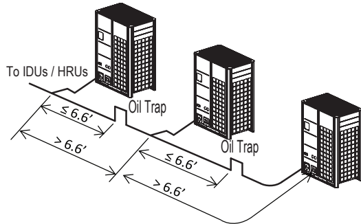
Figure 30: Examples of Inverted Traps.
