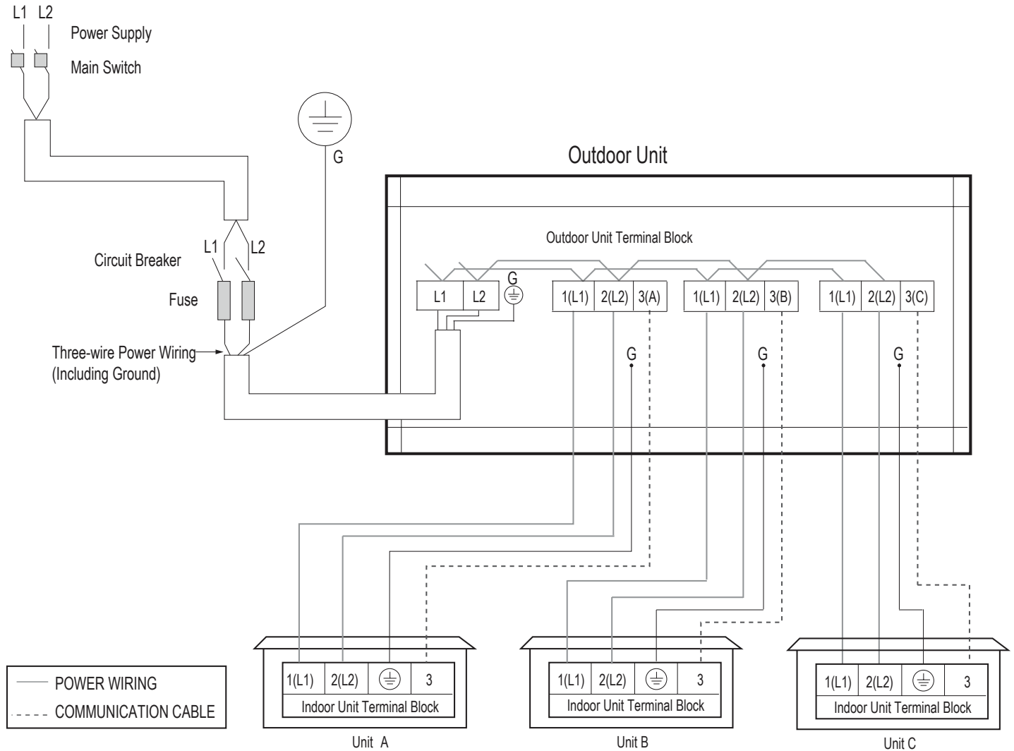
Figure 266: Multi F with LGRED LMU240HHV System Power Wiring and Communications Cable Connections.
