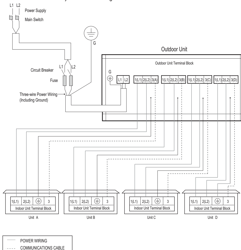
Figure 260: Multi F LMU303HV and LMU363HV System Power Wiring and Communications Cable.
