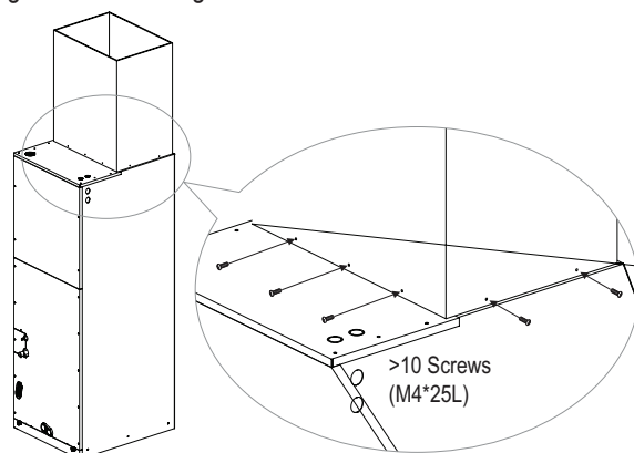
Figure 230: Securing the Ducts to the Unit.
