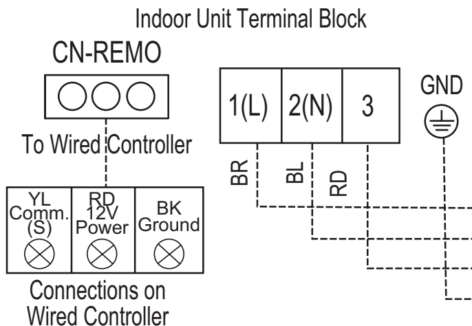
Figure 144:Wired Controller Connections on the Indoor Unit Terminal Block.
