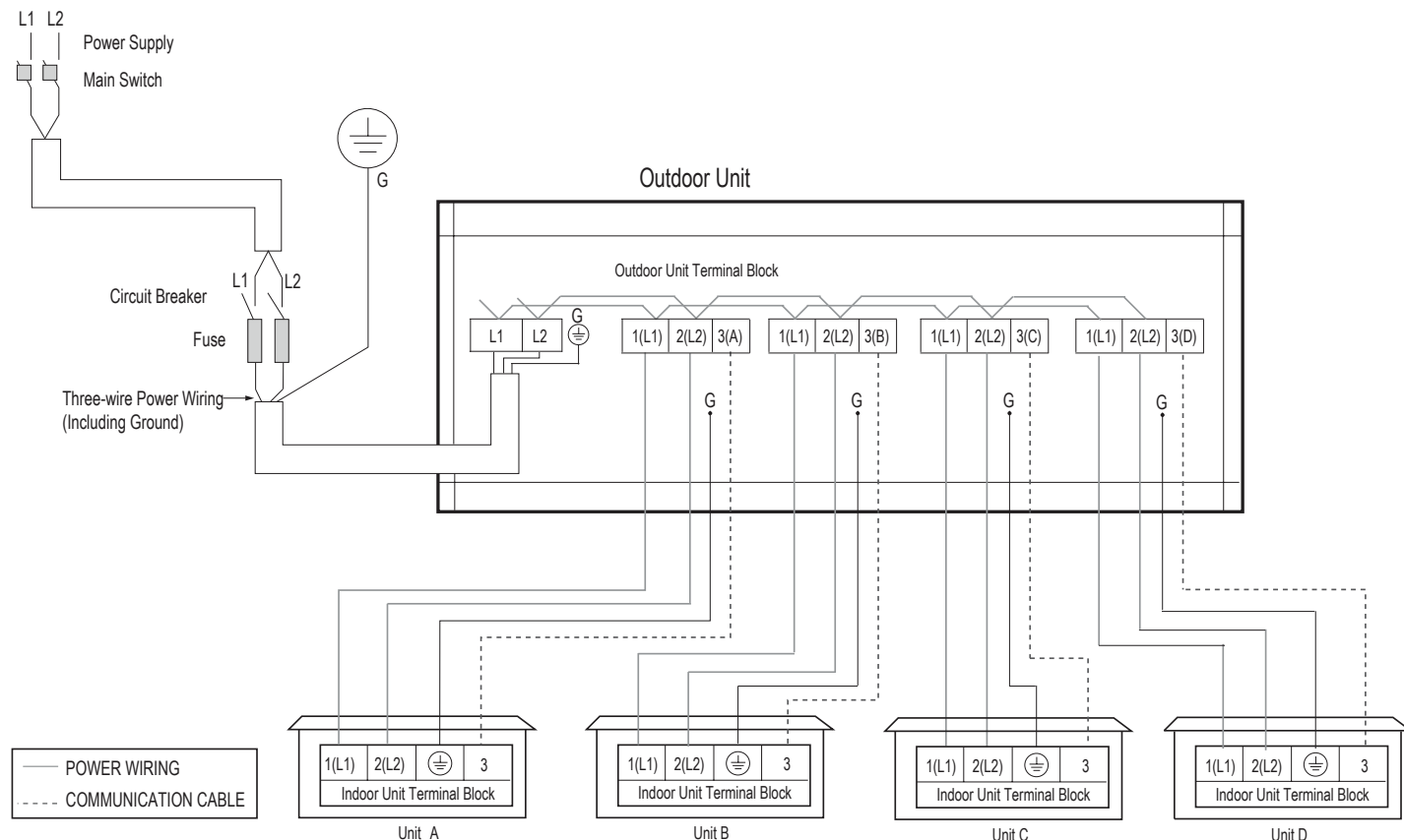
Figure 267: Multi F with LGRED LMU300HHV System Power Wiring and Communications Cable Connections.
