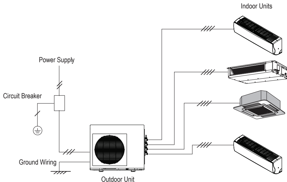
Figure 256: Typical Multi F System General Power / Communications System Schematic.
