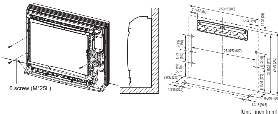
Figure 105:Floor Installation
