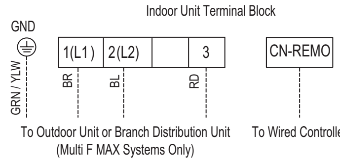
Figure 88:Wired Controller Connection on Indoor Unit Terminal Block— LSN181HSV5 and LMN249HVT Models.
