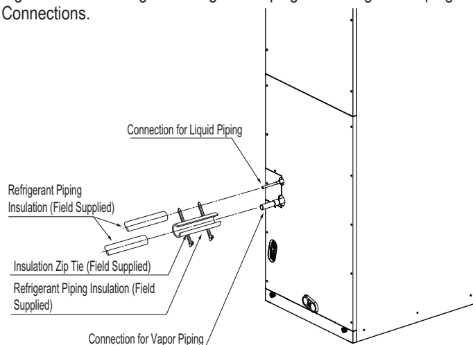
Figure 238: Insulating the Refrigerant Piping and Refrigerant Piping Connections.
