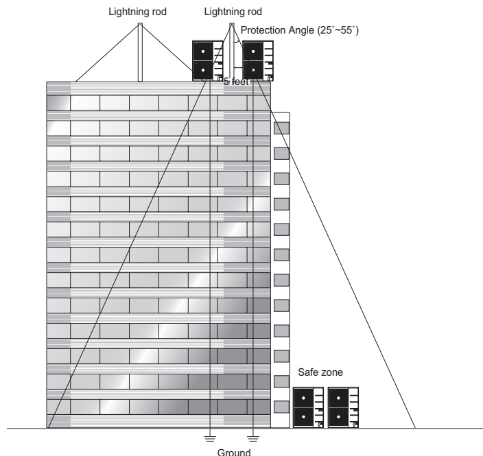
Figure 251: Lightning Protection Diagram.
