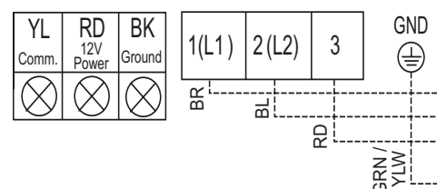
Indoor Unit Terminal Block
