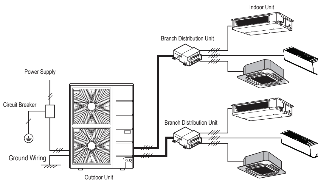
Figure 257: Typical Multi F MAX System General Power / Communications System Schematic.
