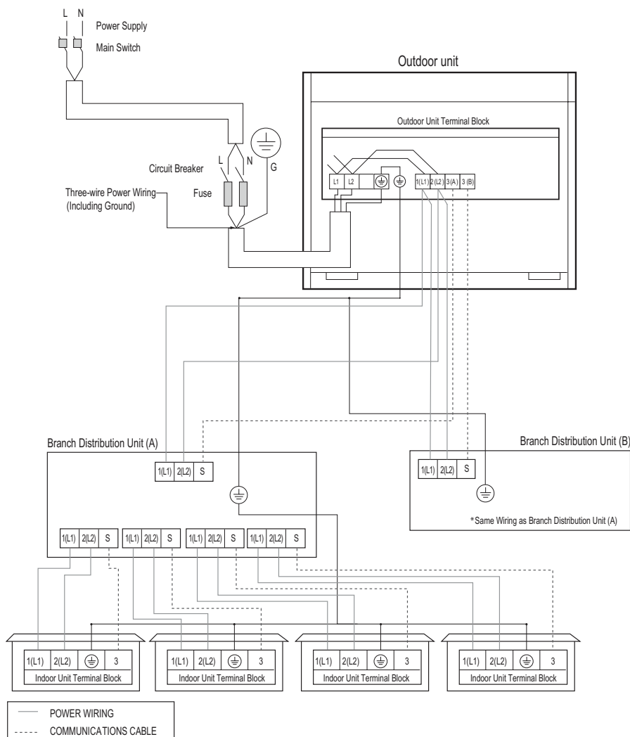
Figure 262: Multi F MAX LMU601HV System Power Wiring and Communications Cable.
