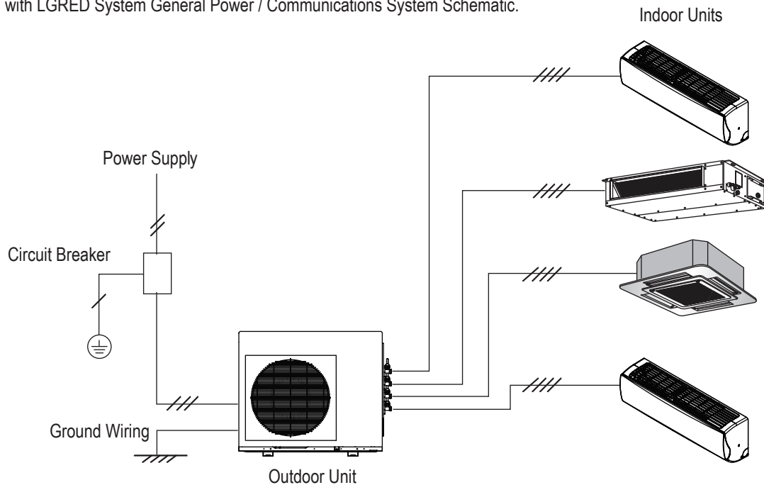
Figure 264: Multi F MAX with LGRED System General Power / Communications System Schematic.
