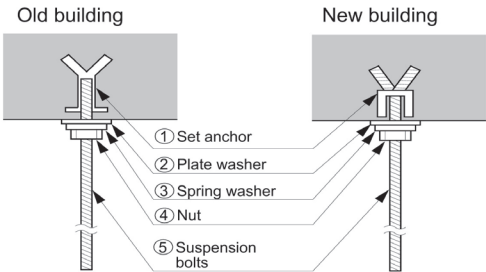
Figure 162: Suspension Bolt Options.
