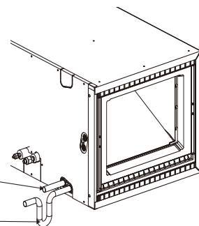
Figure 236: Horizontal Primary and Secondary Drain Layout.
