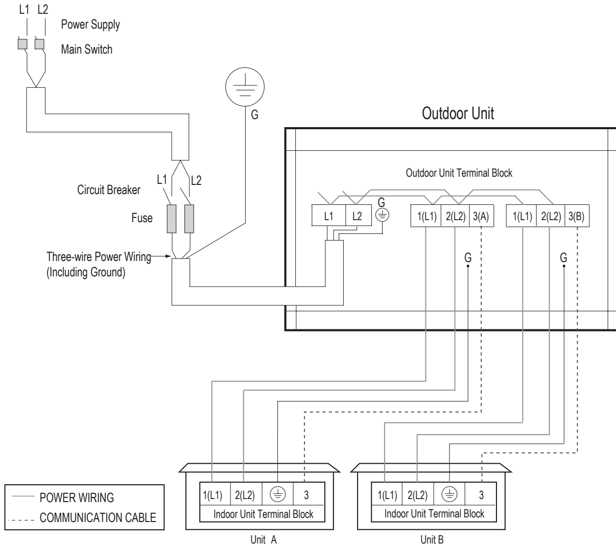
Figure 265: Multi F with LGRED LMU180HHV System Power Wiring and Communications Cable Connections.
