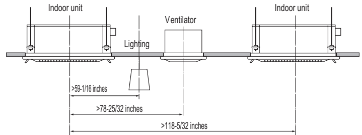
Figure 195: Installing Multiple Indoor Units.
