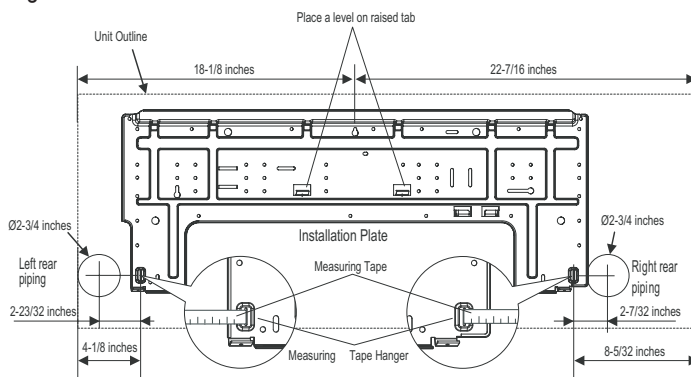
Figure 75: Installation Plate for LSN181HSV5 and LMN249HVT Units.
