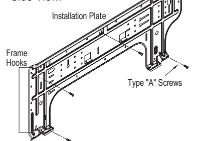
Figure 73: Installation Plate—Side View.
