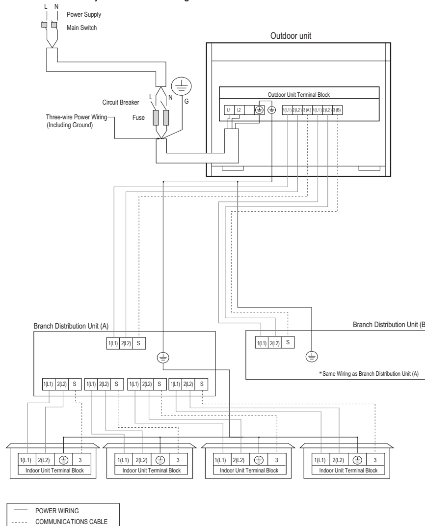
Figure 261: Multi F MAX LMU481HV and LMU541HV System Power Wiring and Communications Cable.
