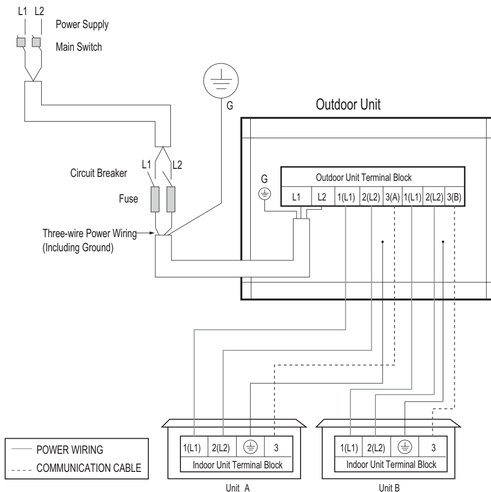
Figure 258: Multi F LMU183HV System Power Wiring and Communications Cable.
