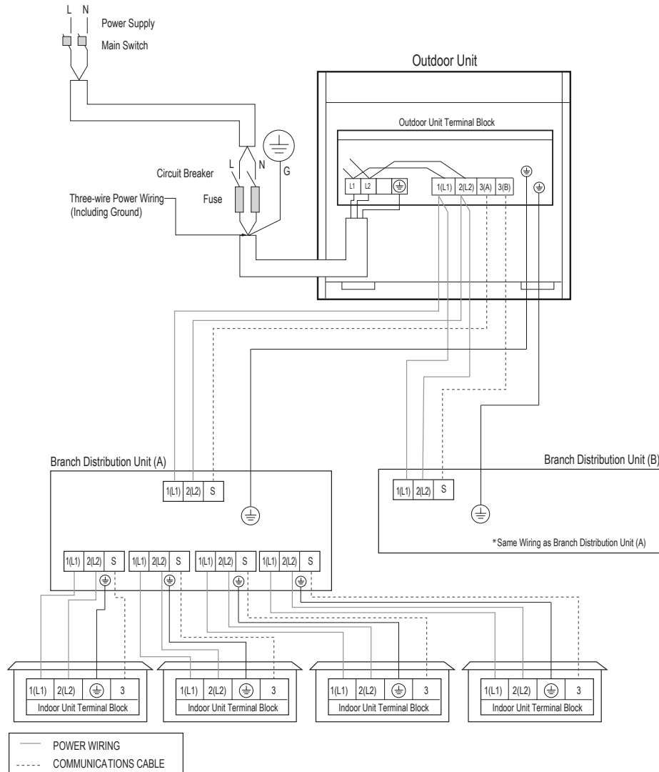
Figure 268: Multi F MAX with LGRED LMU360HHV, LMU420HHV and LMU480HHV System Power Wiring and Communications Cable Connections.
