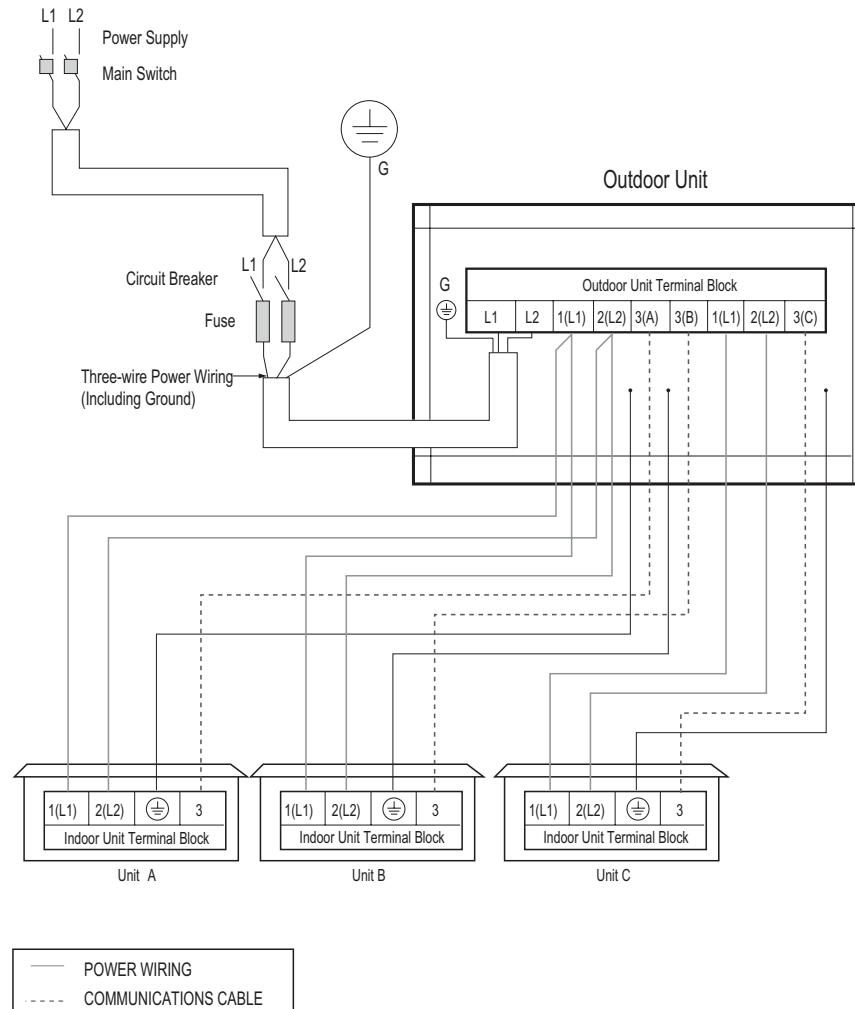
Figure 259: Multi F LMU243HV System Power Wiring and Communications Cable.
