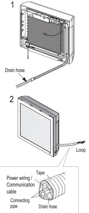
Figure 43: Preparing the Refrigerant / Drain Connections.
