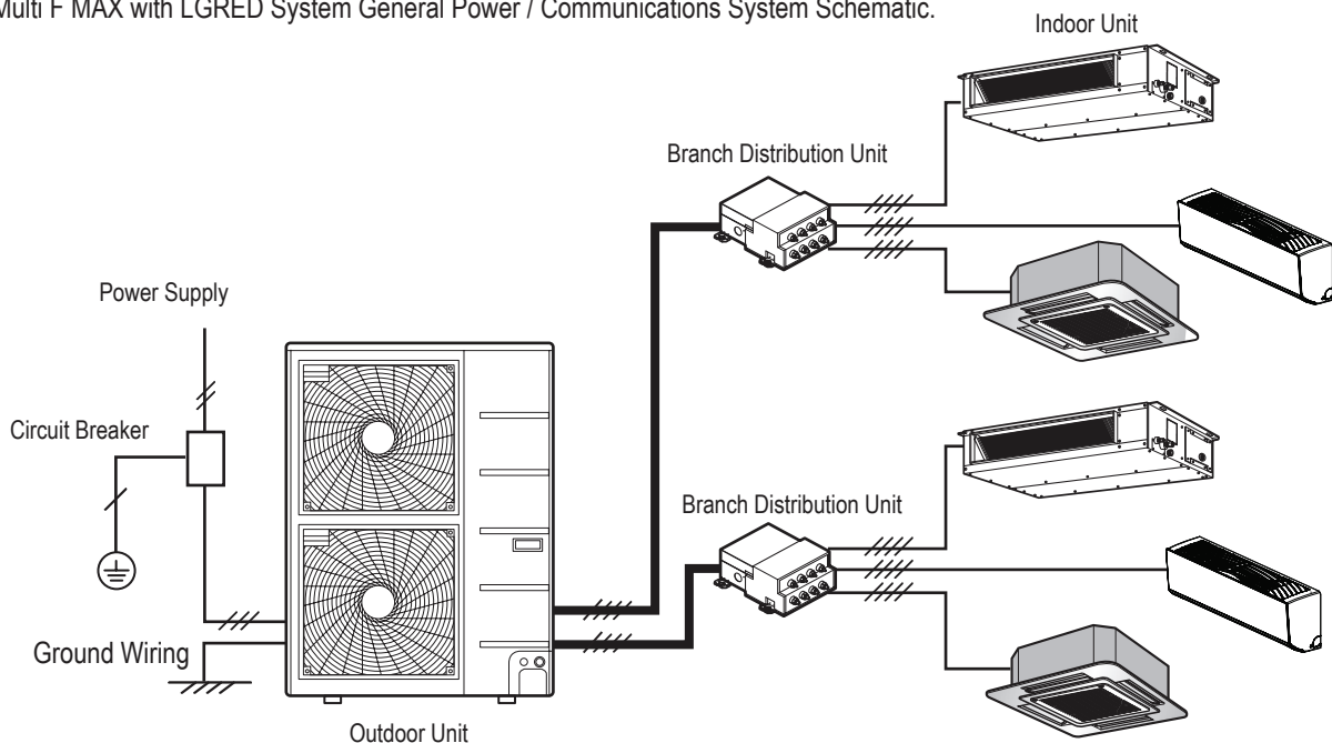
Figure 264: Multi F MAX with LGRED System General Power / Communications System Schematic.
