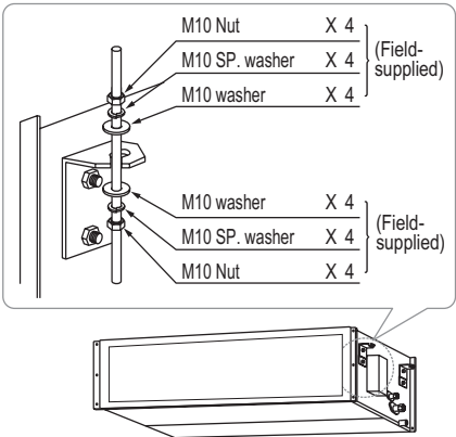
Figure 163: Hanging the Indoor Unit.
