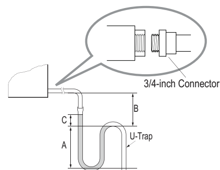
Figure 236: Horizontal Primary and Secondary Drain Layout.
