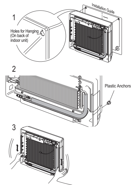
Figure 45: Hanging the Indoor Unit Frame.
