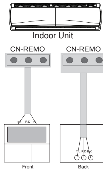
Figure 53: Another Example of Indoor Unit to Zone Controller Connection.
