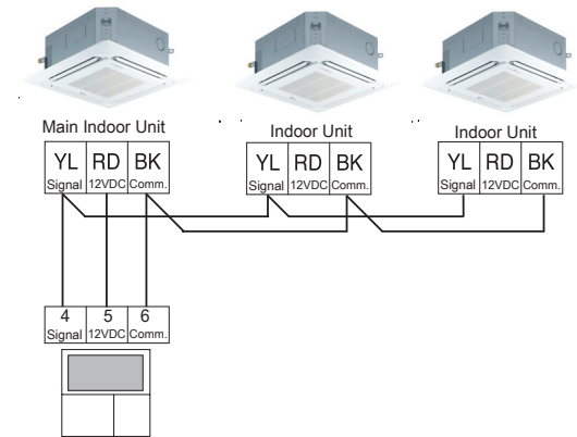
Figure 54: Example of Indoor Unit Group to Zone Controller Connections (Sig-12V-GND [Comm.] Terminal).
