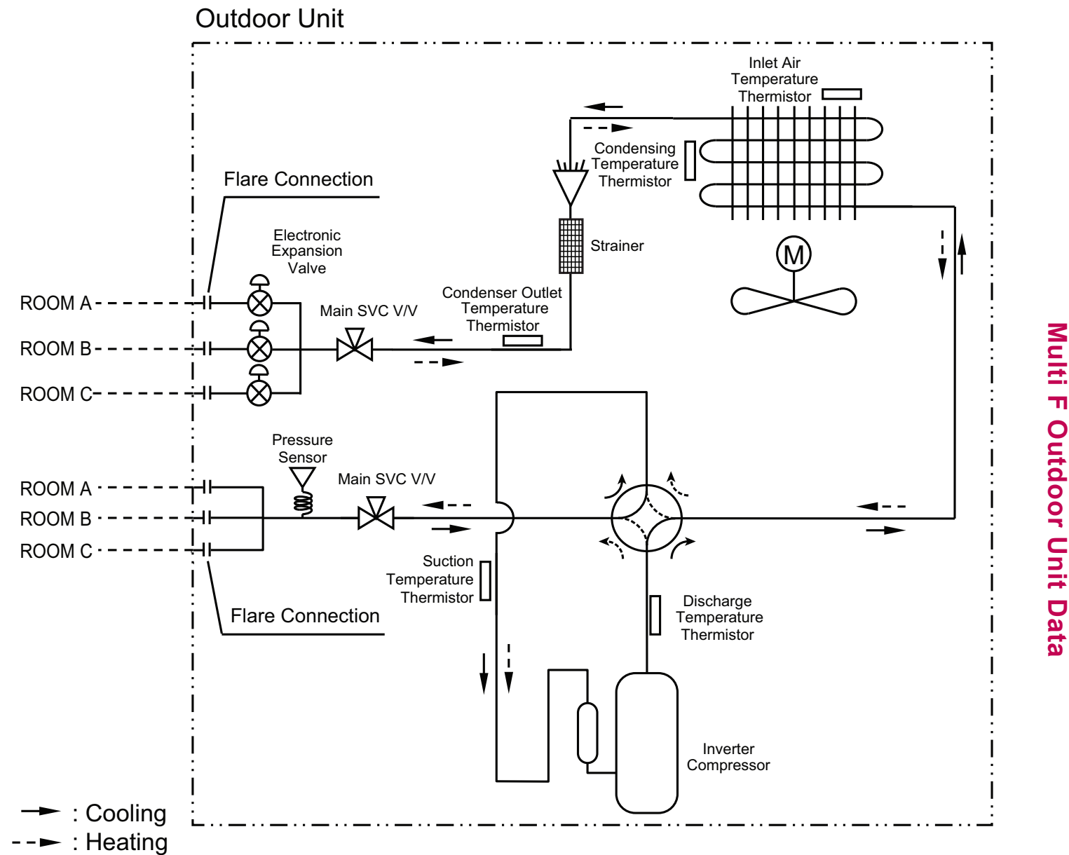
Figure 15: LMU240HV and LMU24CHV Refrigerant Flow Diagram.
