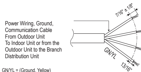
Figure 44: Multi F / Multi F MAX Outdoor and Indoor / Branch Distribution Unit Wiring and Communications Cable Diagram.
