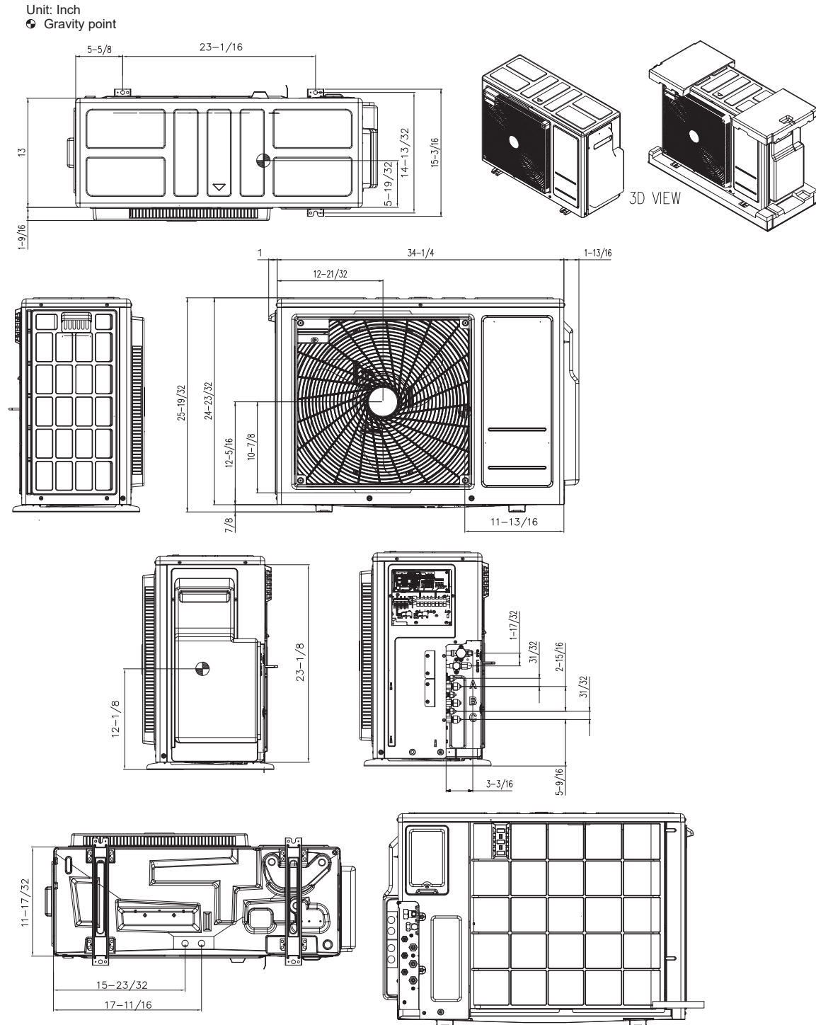
Figure 6: LMU180HV and LMU240HV External Dimensions.
