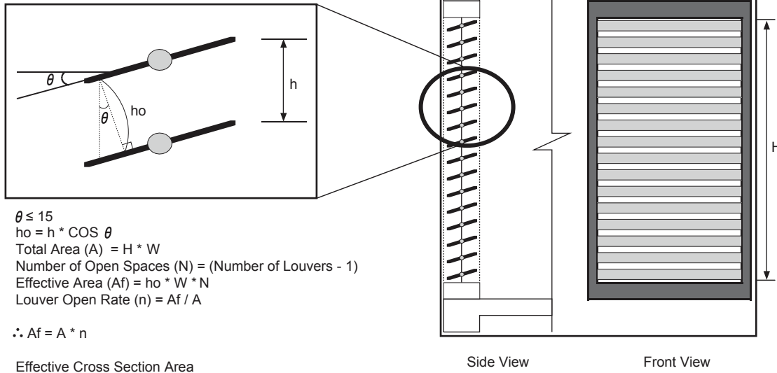
Figure 61: Open Rate by Louver Radian Formula.
