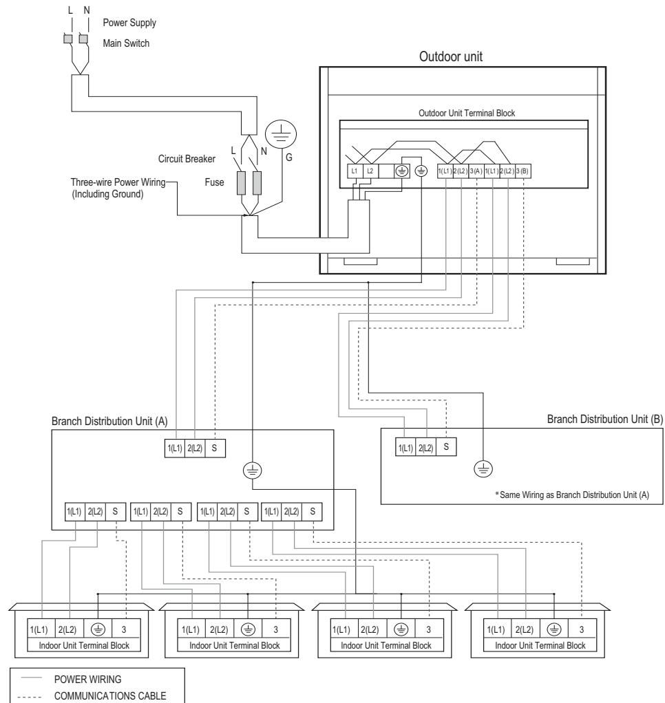
Figure 50: Multi F MAX LMU480HV and LMU540HV System Power Wiring and Communications Cable.
