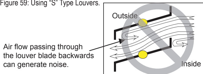
Figure 59: Using “S” Type Louvers.
