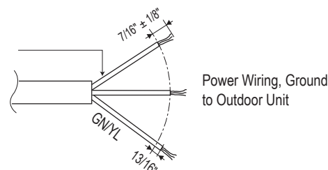
Figure 43: Multi F / Multi F MAX Outdoor Unit Power Wiring.
