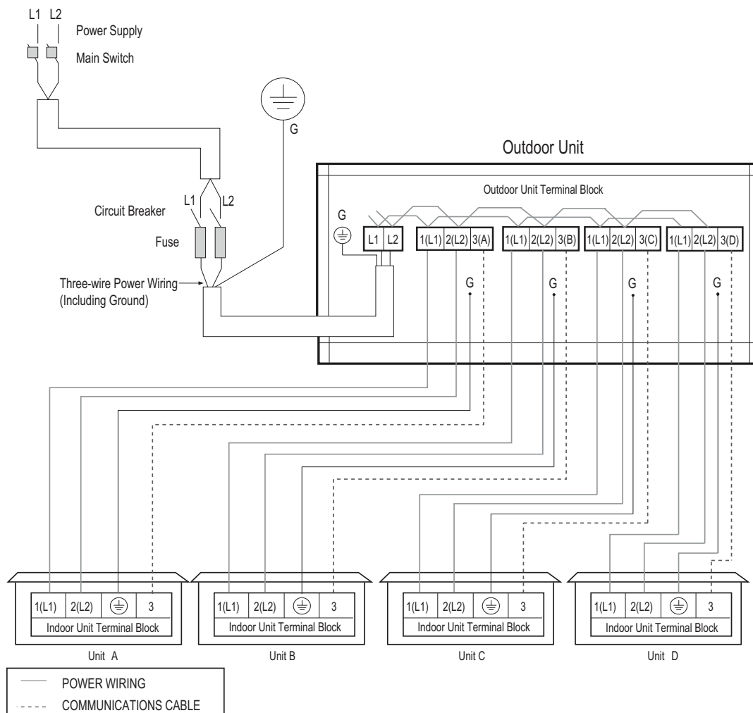
Figure 49: Multi F LMU30CHV and LMU36CHV System Power Wiring and Communications Cable.
