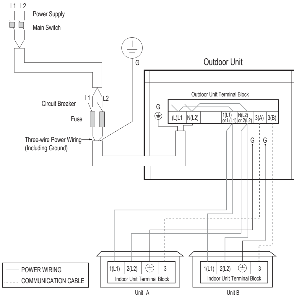
Figure 47: Multi F LMU180HV and LMU18CHV System Power Wiring and Communications Cable.
