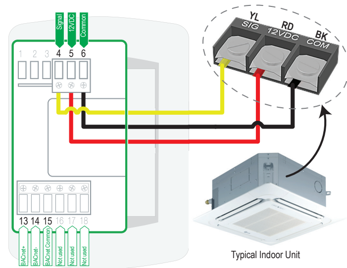
Figure 52: One Example of Indoor Unit to Zone Controller Connection.
