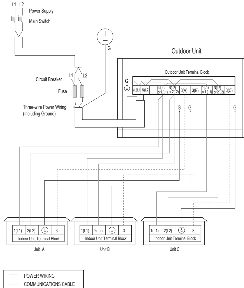
Figure 48: Multi F LMU240HV and LMU24CHV System Power Wiring and Communications Cable.
