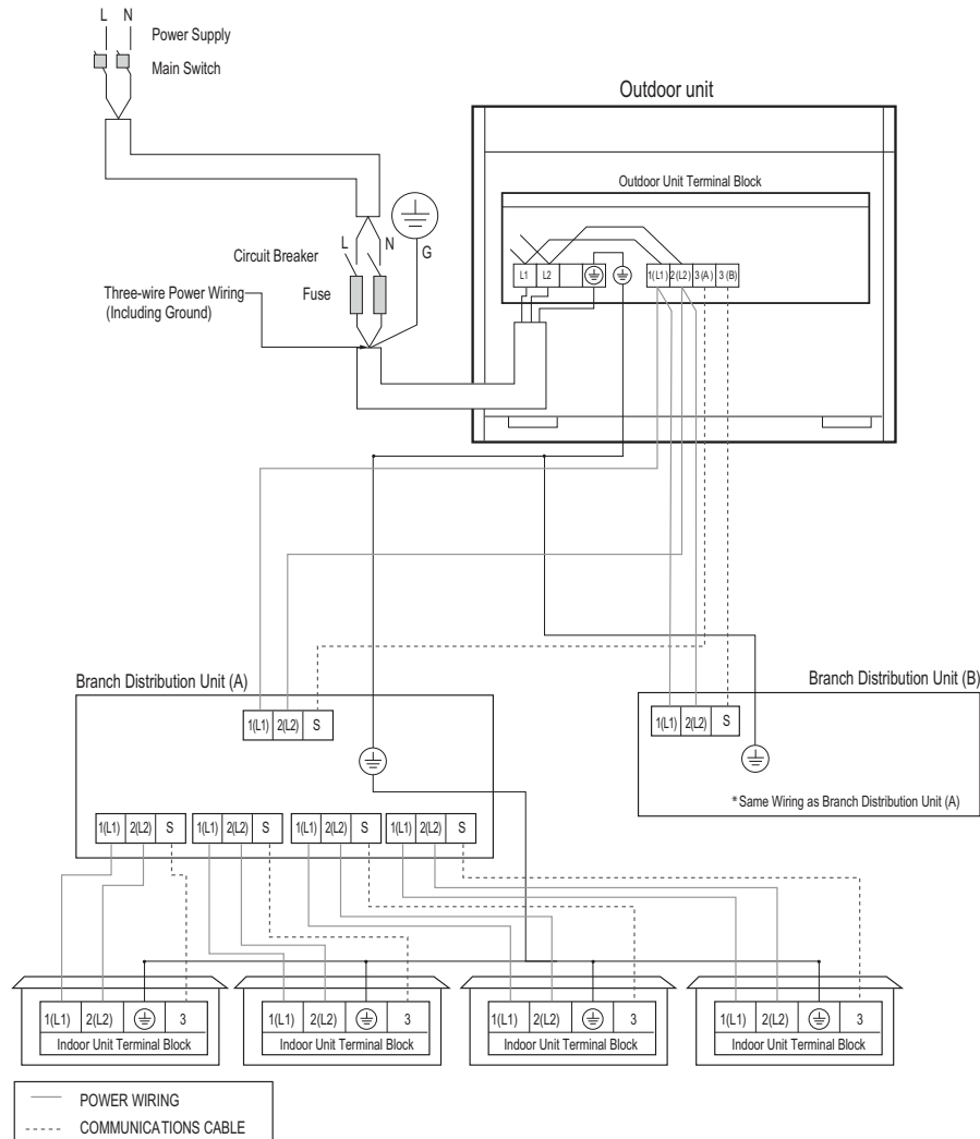
Figure 51: Multi F MAX LMU600HV System Power Wiring and Communications Cable.
