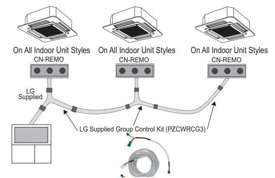
Figure 55: Example of Indoor Unit Group to Zone Controller Connections (CN-REMO).
