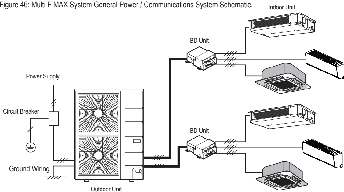
Figure 46: Multi F MAX System General Power / Communications System Schematic.
