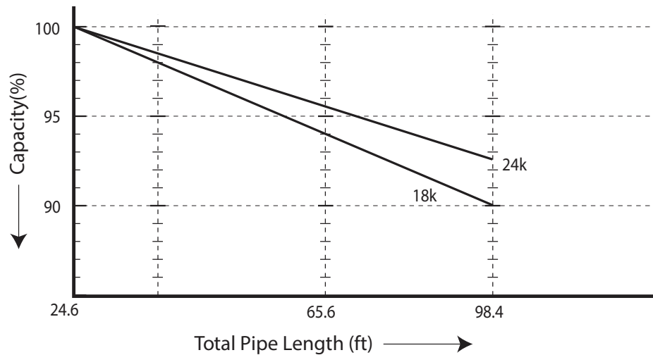
Figure 10: Heating Capacity Coefficient Factor
