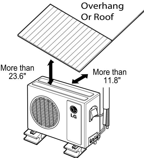
Figure 17: Art Cool Mirror Outdoor Unit Under Roof/Overhang
