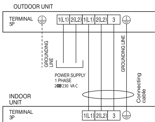
Figure 32: Terminal Block Wiring Diagram LAU090HSV2, LAU120HSV2
