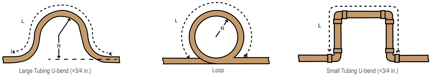
Figure 19: Coiled Expansion Loops and Offsets
