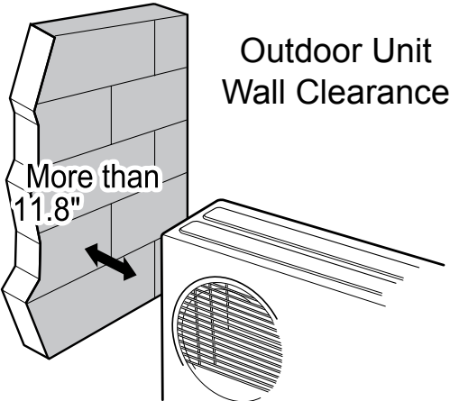
Figure 16: Art Cool Mirror Outdoor Unit Next to Wall - Clearance
