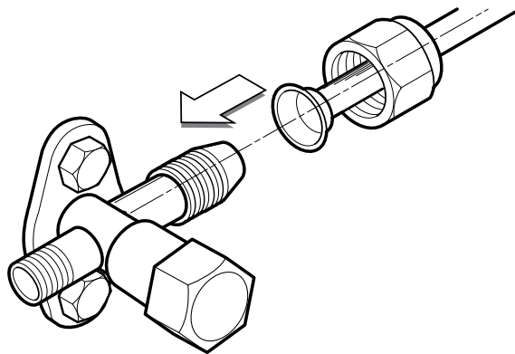
Figure 27: Pipe Attachment
