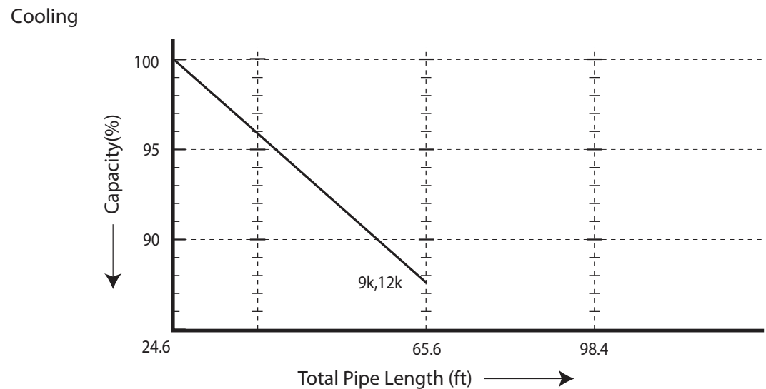
Figure 7: Cooling Capacity Coefficient Factor
