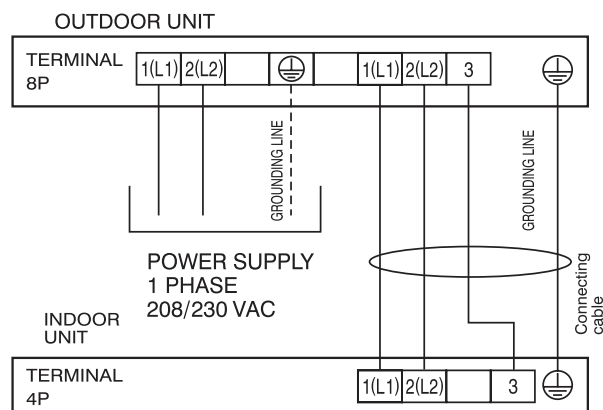
Figure 33: Terminal Block Wiring Diagram LAU180HSV2, LAU240HSV2
