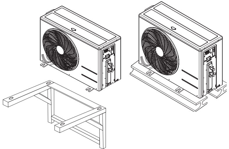
Figure 14: Outdoor Unit—Mounting Methods
