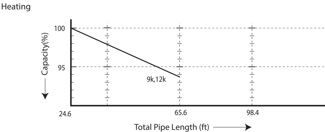
Figure 8: Heating Capacity Coefficient Factor
