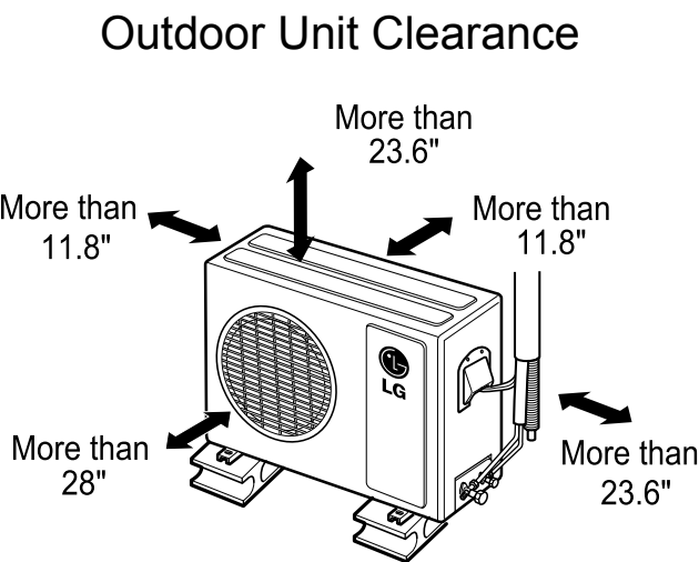
Figure 15: Art Cool Mirror Outdoor Unit Clearance
