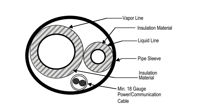
Figure 25: Typical Arrangement of Refrigerant Pipe and Cable(s) in a Utility Conduit
