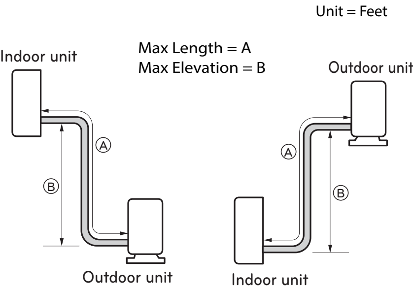
Figure 18: Art Cool Mirror System Layout
