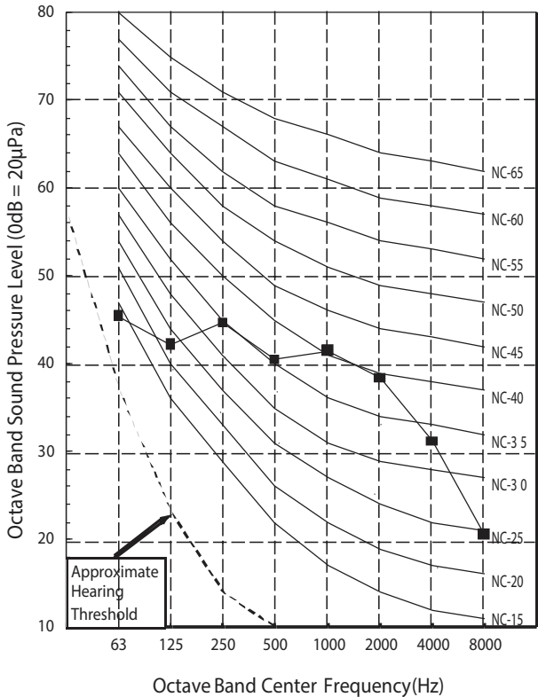
Figure 4: LAU180HSV2/LAU240HSV2
