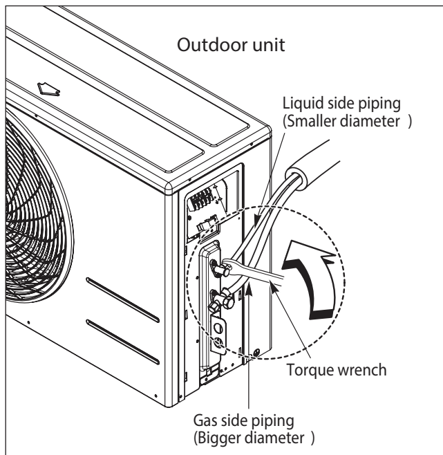
Figure 28: Heat Pump Outdoor Unit Piping Connection
