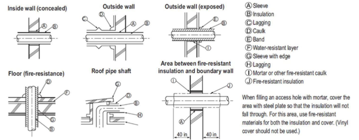
Figure 24: Pipe Sleeve Options
