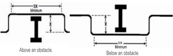
Figure 20: Installing Piping Above and Below an Obstacle
