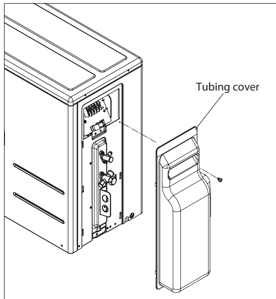
Figure 26: Outdoor Unit Connection Cover Removal
