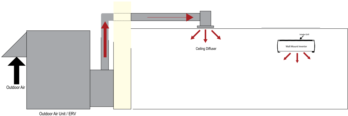
Figure 11: Decoupled Dedicated Outdoor System Diagram
