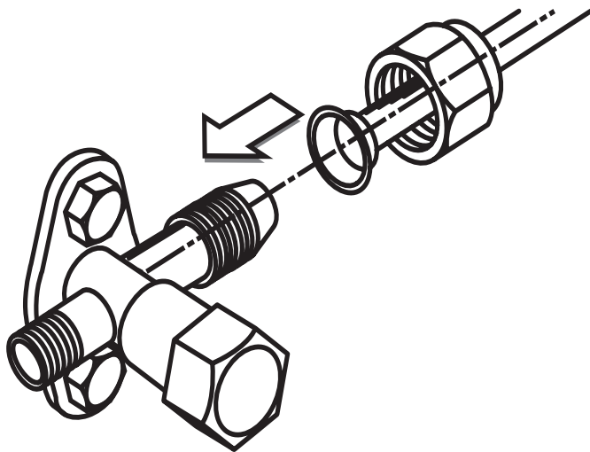
Figure 38: Pipe Attachment
