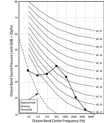
Figure 15: LSN300HLV
