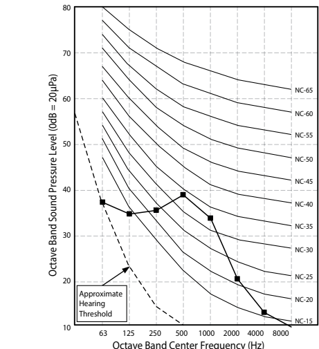
Figure 16: LSN360HLV
