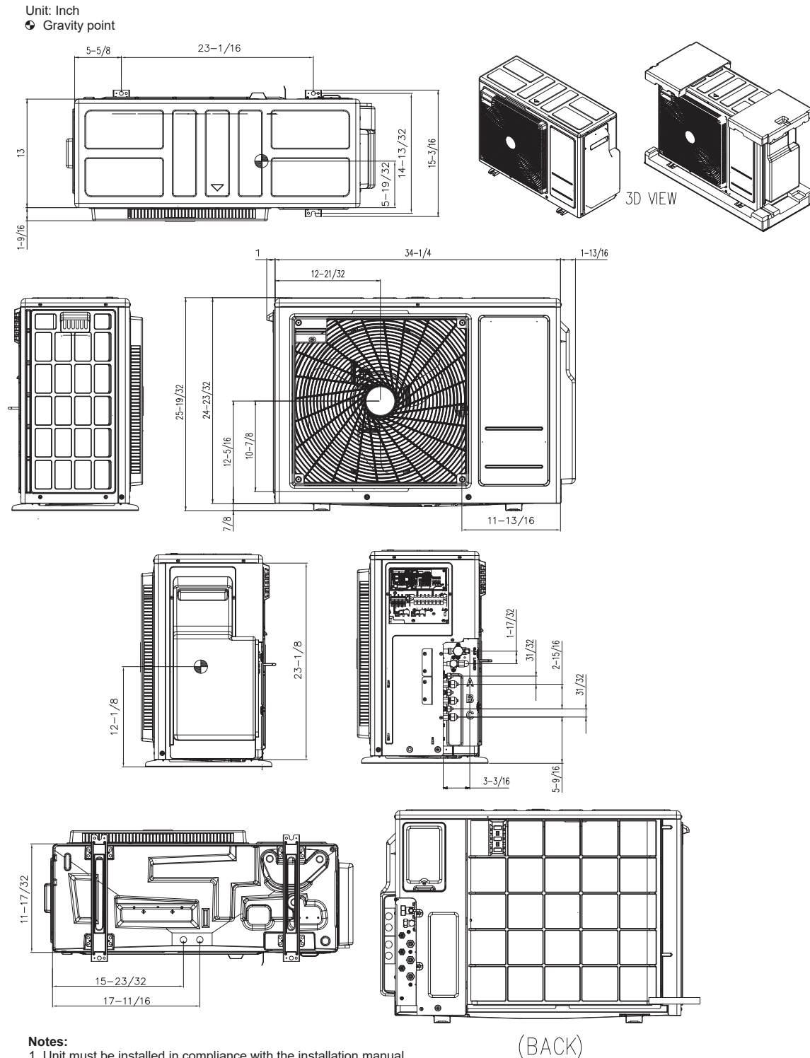
Figure 6: LMU183HV and LMU243HV External Dimensions.
