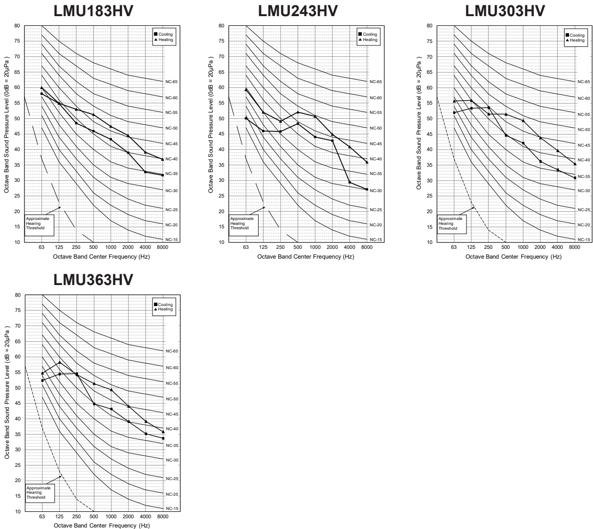
Figure 15: Sound Pressure Level Diagrams.
