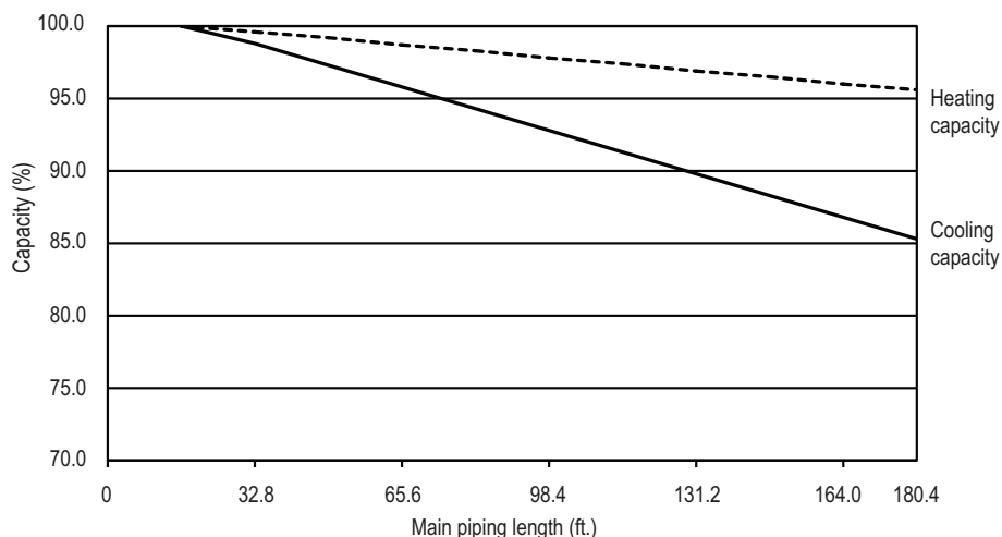
Figure 3: Multi F MAX Outdoor Unit to Branch Distribution Unit Refrigerant Line Length Derate Chart.
