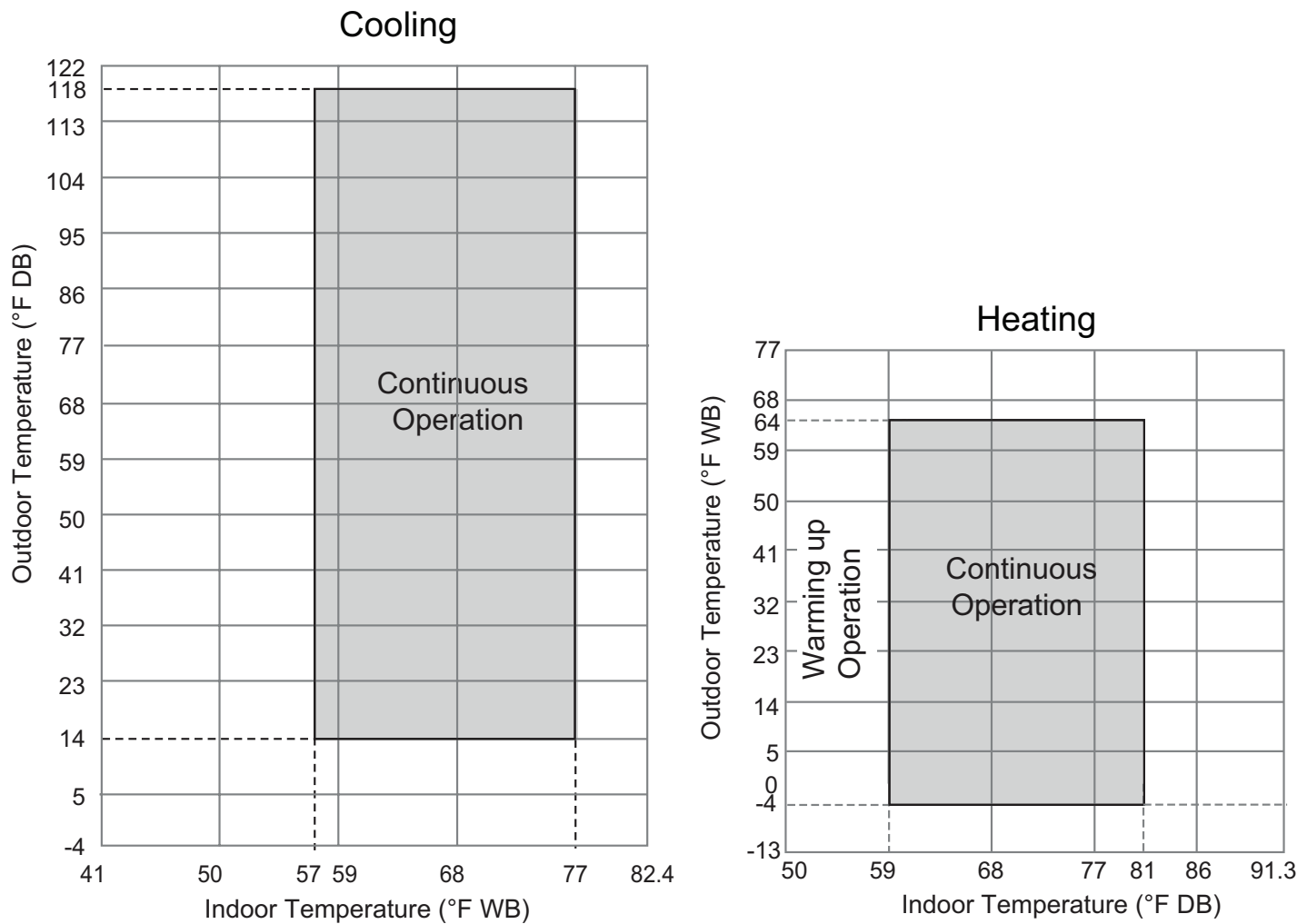
Figure 17: Cooling and Heating Operation Ranges.
