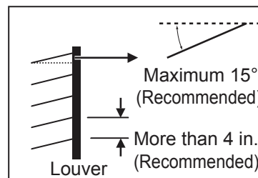
Figure 59: Louver Recommendations.
