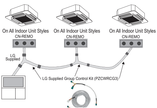
Figure 56: Example of Indoor Unit Group to Zone Controller Connections (CN-REMO).
