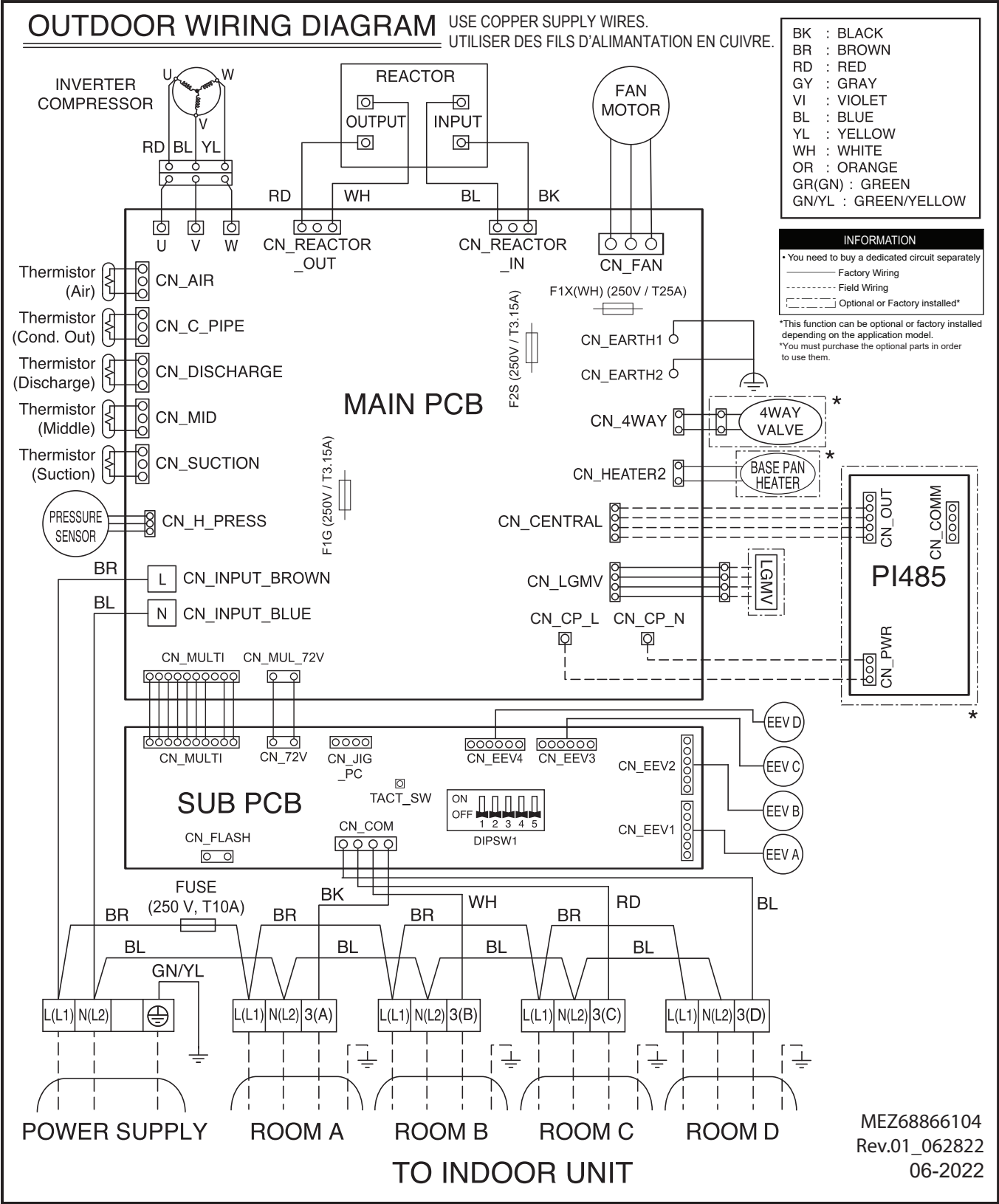
Figure 10: LMU303HV and LMU363HV Wiring Diagram.
