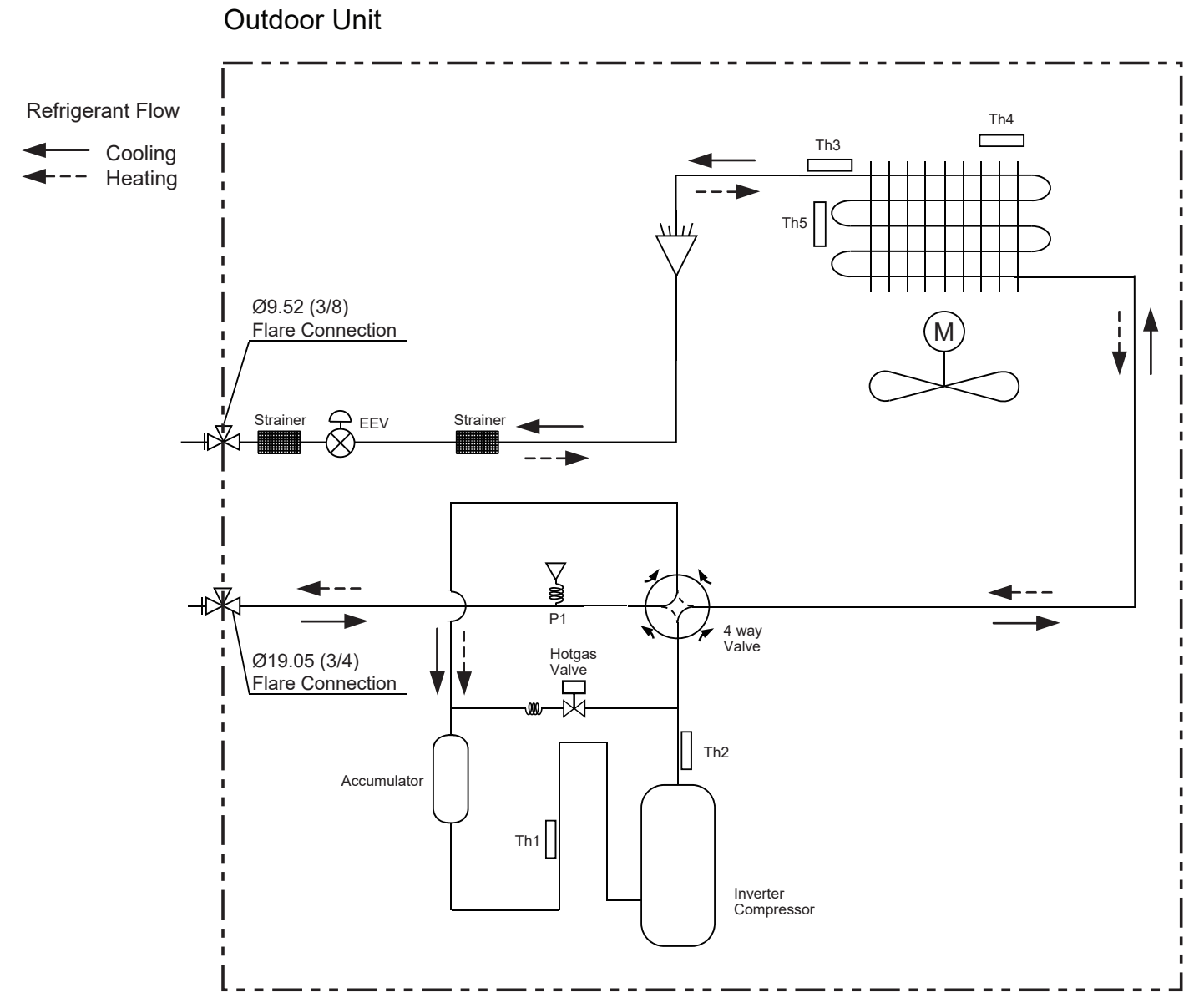
Figure 25: LMU481HV and LMU541HV Refrigerant Flow Diagram.
