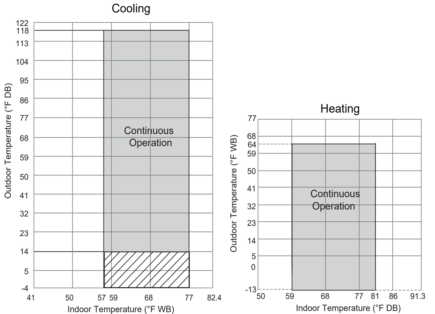
Figure 23: Multi F MAX with LGRED Cooling and Heating Operation Ranges.
