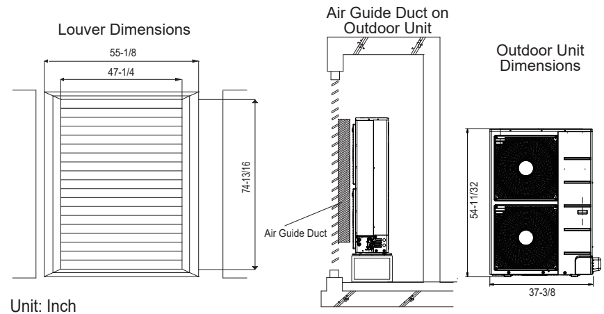
Figure 54: Example of Installing Outdoor Unit Indoors.
