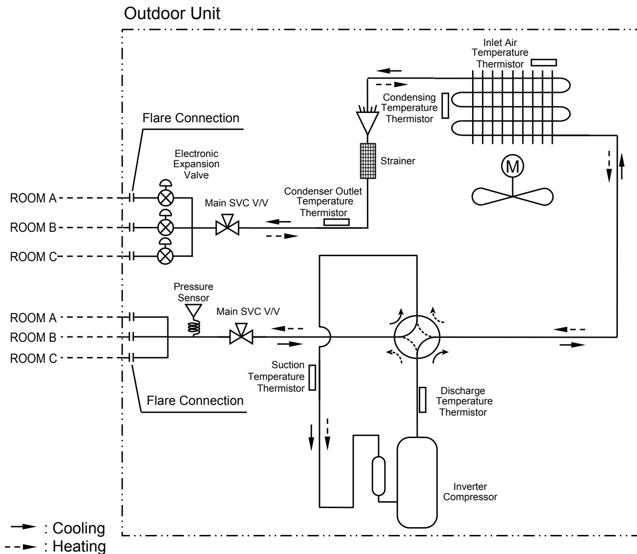
Figure 10: LMU240HHV Refrigerant Flow Diagram.
