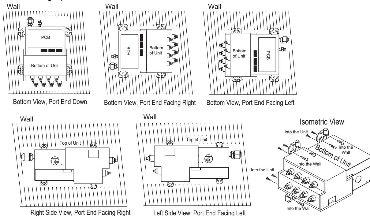
Figure 36: Unacceptable Branch Distribution Unit Orientation.
