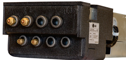
Figure 25: PMBD3630 Three-Port Branch Distribution Unit.
