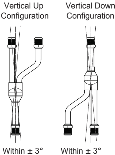
Figure 33: Y-branch Installation Alignment Specification.
