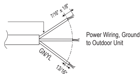
Figure 37: Multi F / Multi F MAX with LGRED Outdoor Unit Power Wiring.
