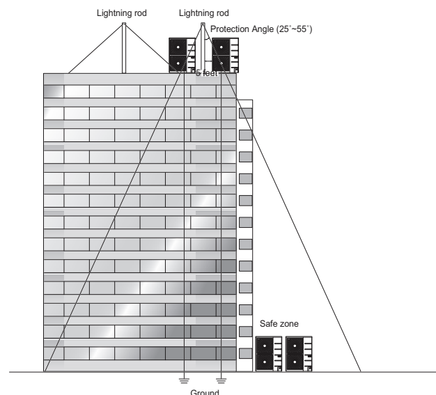
Figure 49: Lightning Protection Diagram.
