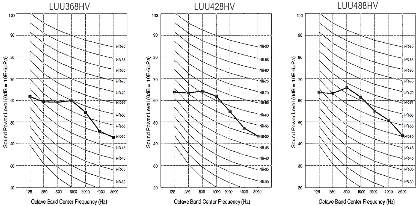
Figure 19: LUU368HV , LUU428HV, LUU488HV Sound Power Level Diagrams.
