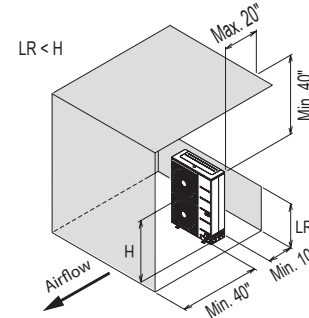
Figure 50: Proper Outdoor Unit Placement and Clearances.
