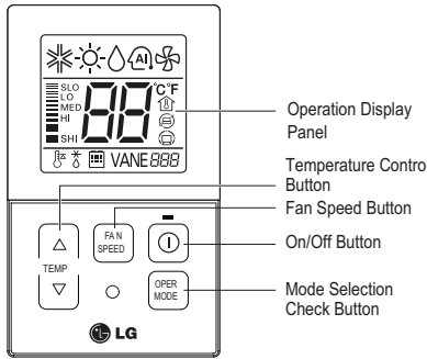
Figure 30: PQRCVCL0QW Wired Controller.
