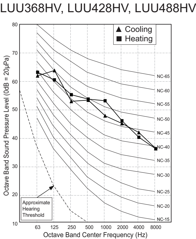
Figure 17: LUU368HV, LUU428HV, LUU488HV Sound Pressure Level Diagram.
