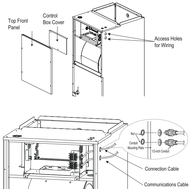
Figure 27: Connecting the Power Wiring and Communications Cable.
