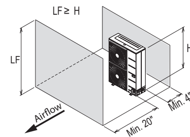
Figure 51: Proper Outdoor Unit Placement and Clearances, continued.
