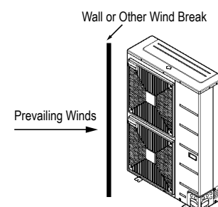
Figure 46: Wind Break.
