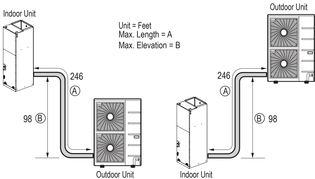
Figure 55: Typical LV360HV4, LV480HV and LV488HV System Layout.
