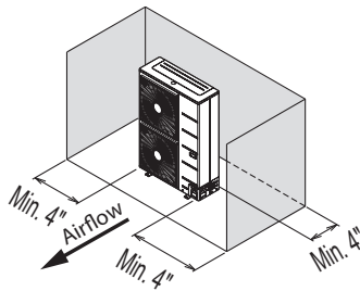
Figure 51: Proper Outdoor Unit Placement and Clearances, continued.
