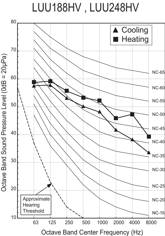
Figure 16: LUU188HV , LUU248HV Sound Pressure Level Diagram.
