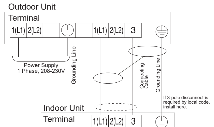
Figure 19: HLV3 Power / Communication System Diagram For Wiring Lengths GREATER THAN 130 Feet.
