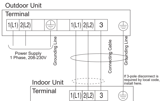
Figure 18: Typical HLV3 Power / Communication System Diagram For Wiring Lengths Up to 130 Feet..
