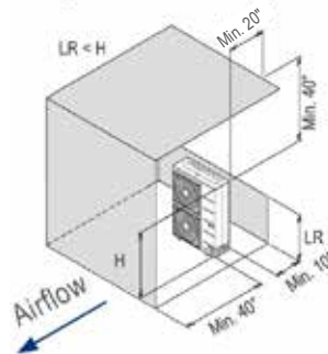
Figure 20: Single Unit—high rear and front walls with no side walls
