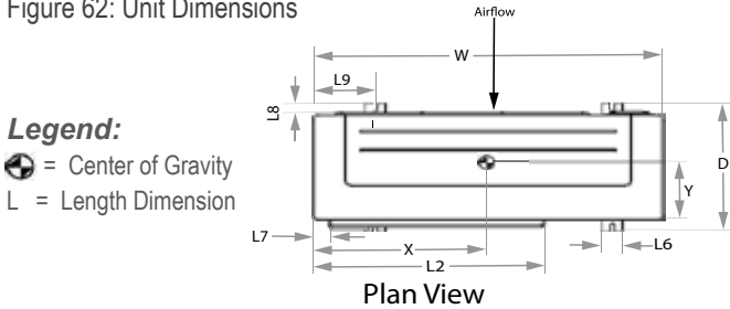
Figure 62: Unit Dimensions
