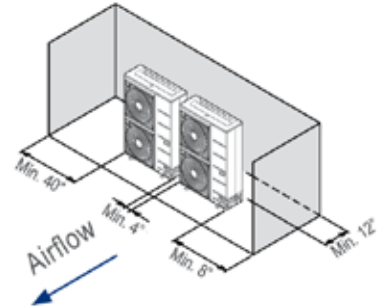
Figure 21: Side by Side—high rear and side walls
