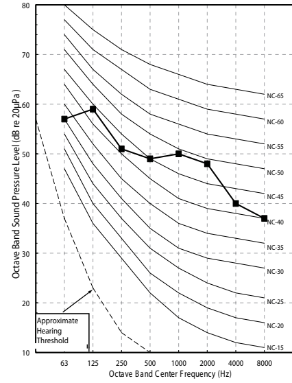
Figure 6: ARUN053GS2 Heating
