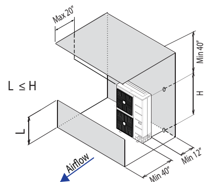
Figure 24: Single Unit—high rear wall and low front wall with building overhang and no side walls
