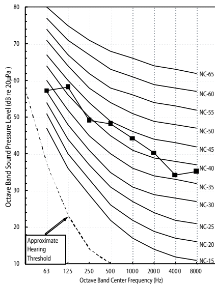
Figure 4: ARUN036GS2 (Heating)
