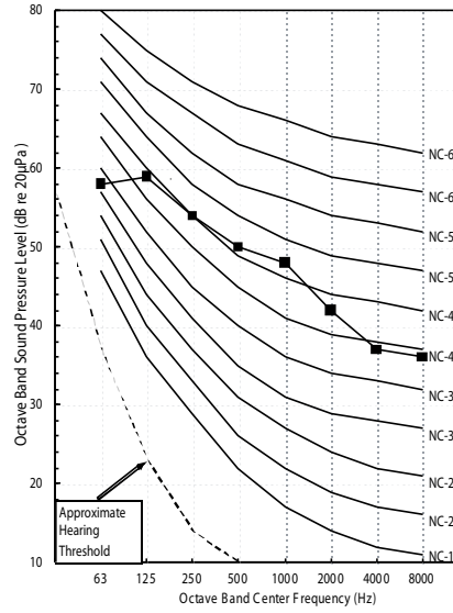
Figure 5: ARUN047GS2 (Heating)
